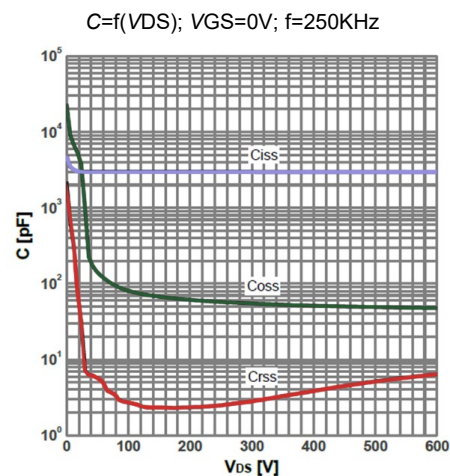
Figure 12: Typ. capacitances
