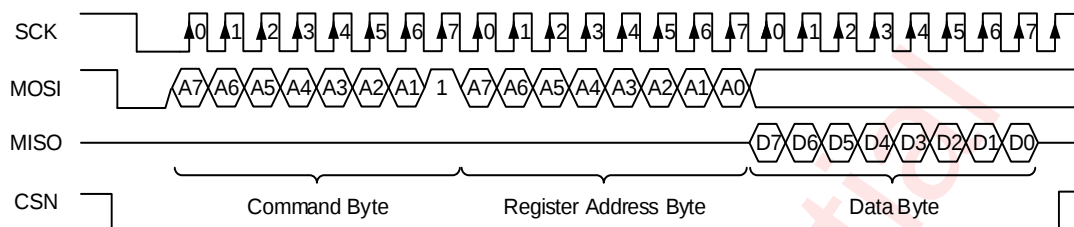
Figure 13 SPI Read from AW20144S (Typical)
