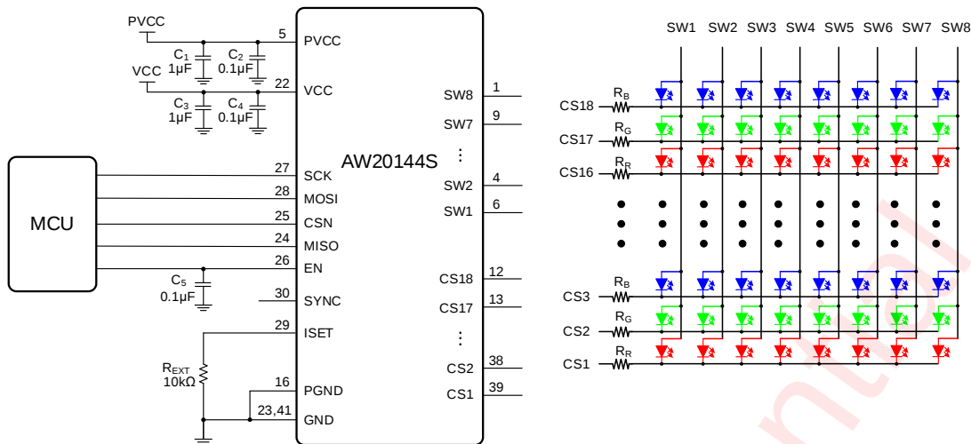
Figure 5 Typical Application Circuit (RGB)
