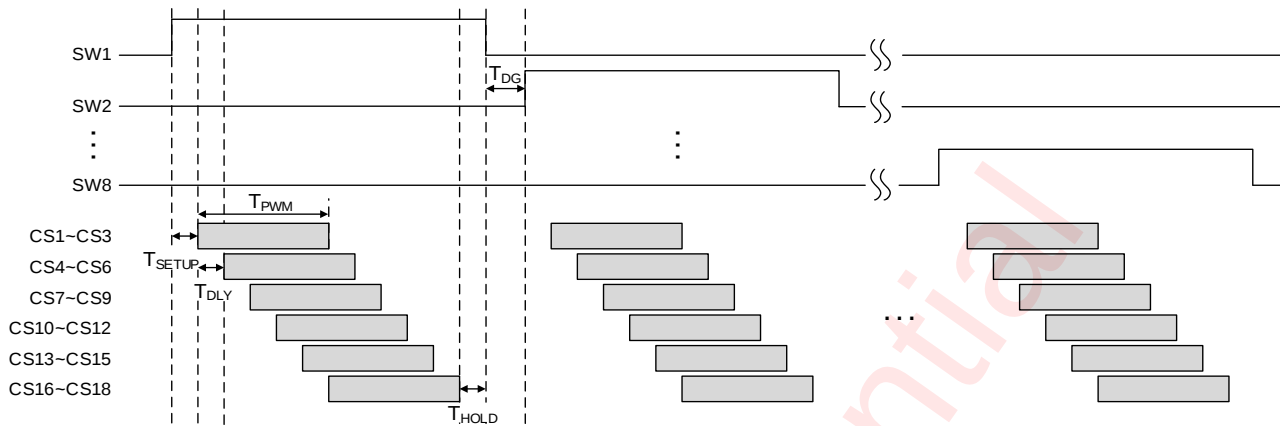
Figure 19 Scanning Timing
