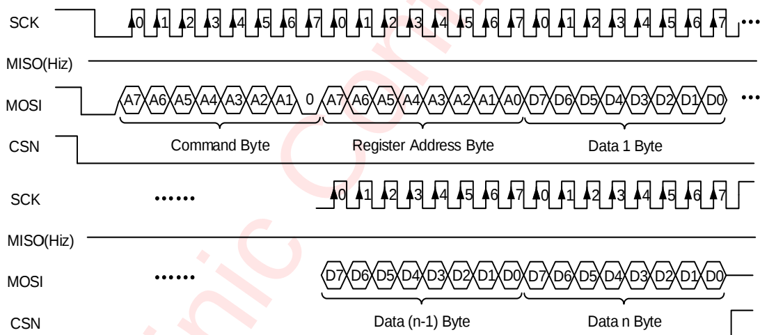
Figure 12 SPI Writing to AW20144S (Automatic Address Increment)
