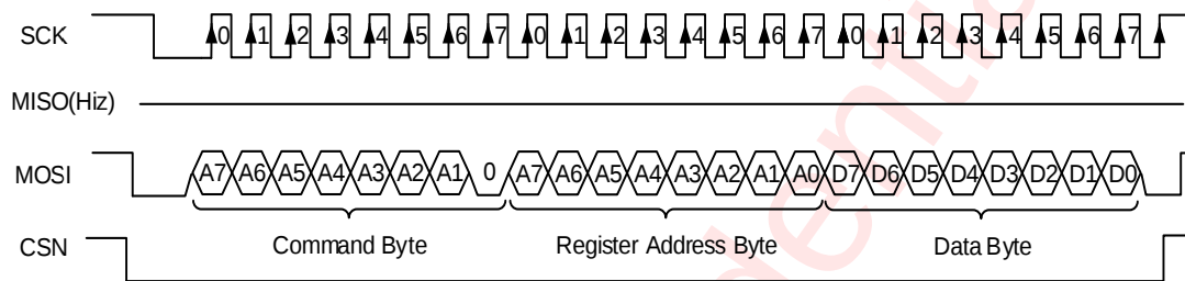
Figure 11 SPI Writing to AW20144S (Typical)
