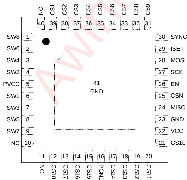
Figure 2 Pin Configuration and Top Marking
