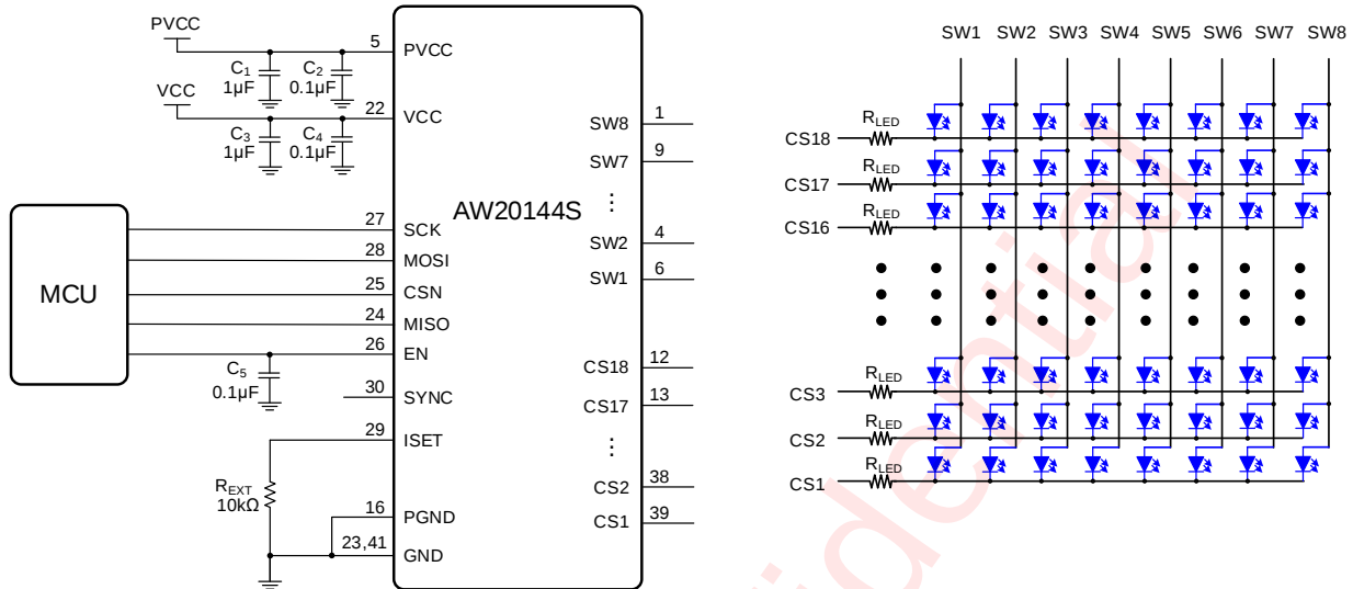
Figure 1 AW20144S Application Circuit
