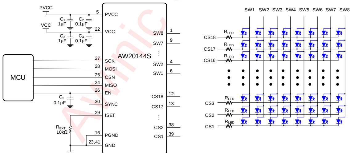
Figure 4 Typical Application Circuit
