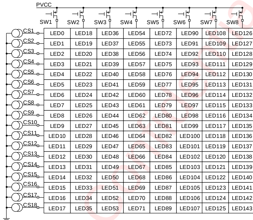
Figure 16 LED Location
