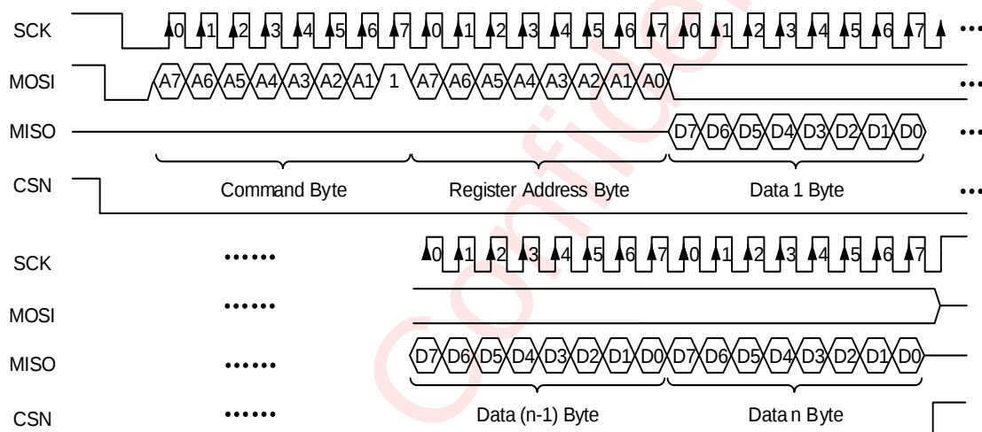
Figure 14 SPI Read from AW20144S (Automatic Address Increment)
