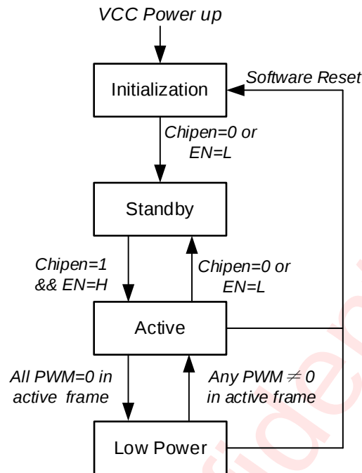
Figure 10 AW20144S Operating Mode Transition
