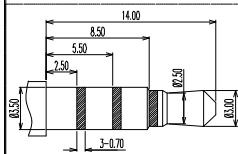
Ø3.50mm 4 POLE PLUG DETAIL
