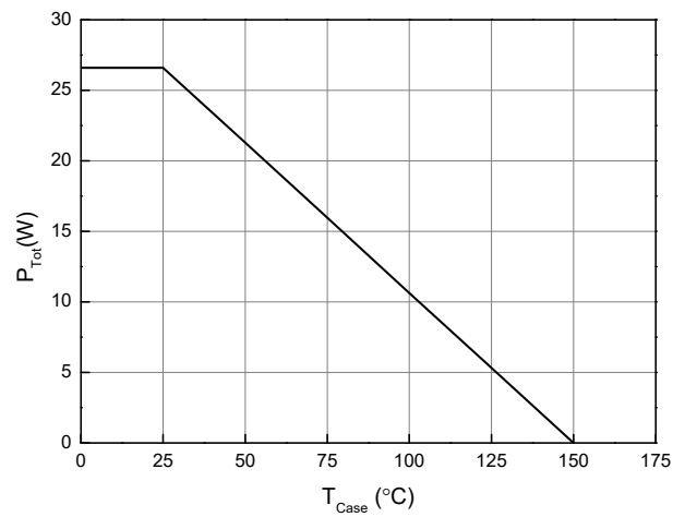
Figure 9. Power Dissipation
