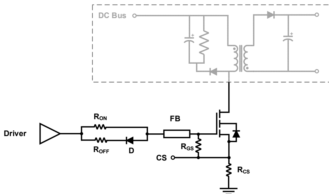
Figure 13. Simplified flyback schematic
