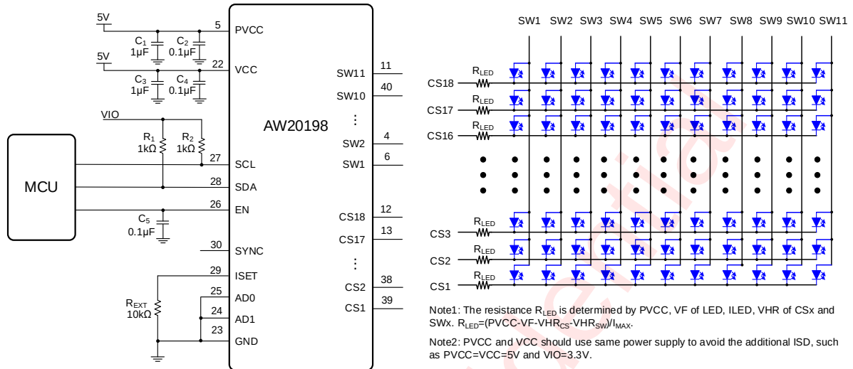
Figure 1 AW20198 Application Circuit
