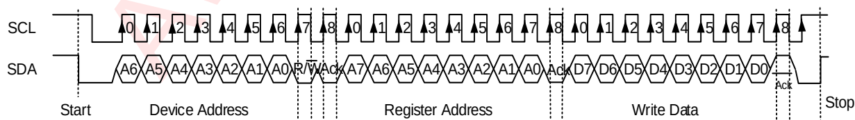
Figure 13 I²C Write Byte Cycle
