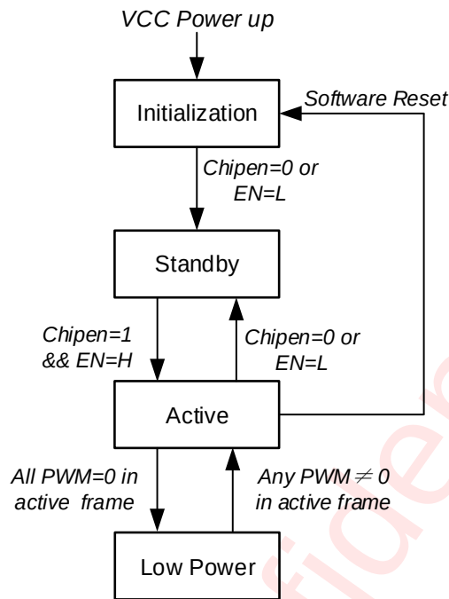
Figure 9 AW20198 Operating Mode Transition
