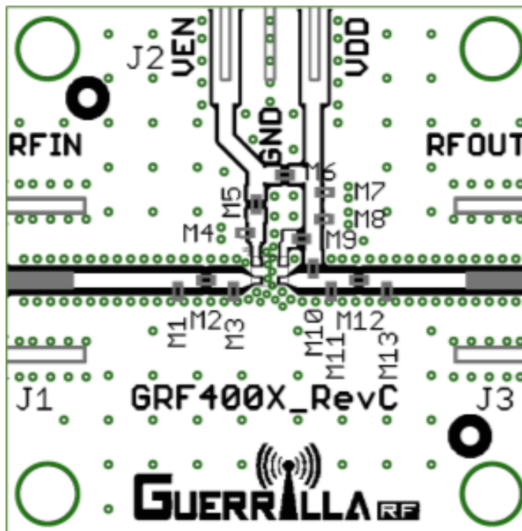
GRF2042 Evaluation Board Assembly Diagram
