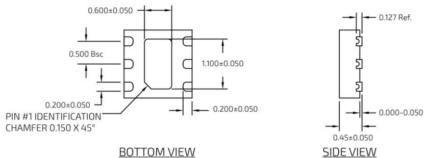
DFN-6 1.5 x 1.5 mm DFN-6 Package Dimensions
