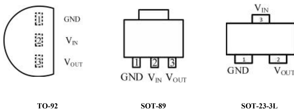
Figure 2.HT75XX Pin
