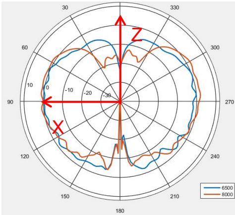
2D-Phi=0
