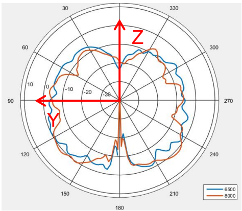
2D-phi=90
