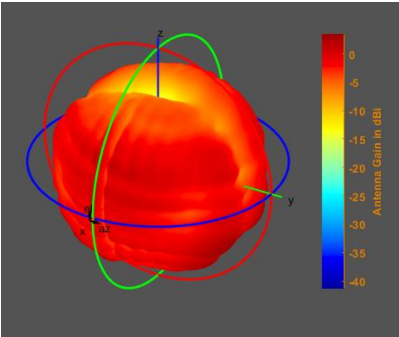
3D Gain Pattern (CH9)
