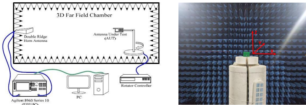
Fig.3 FAR-field Chamber
