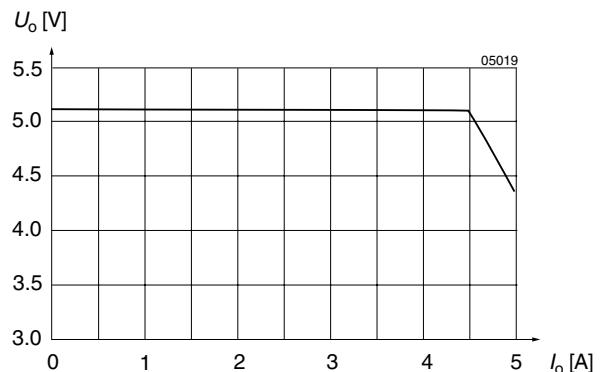
Fig. 7 U_o versus I_o (typ) of units with U_o = 5.1 V.
