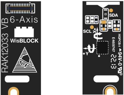
Figure 1: RAK12033 WisBlock 6-Axis Accelerometer Sensor Module
