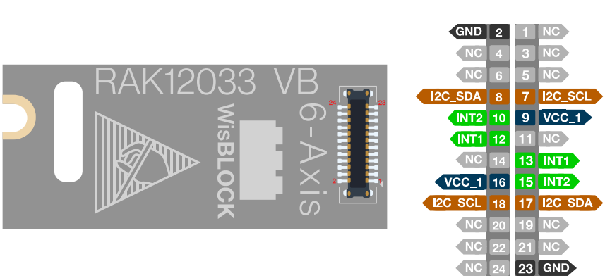
Figure 2: RAK12033 pinout diagram
