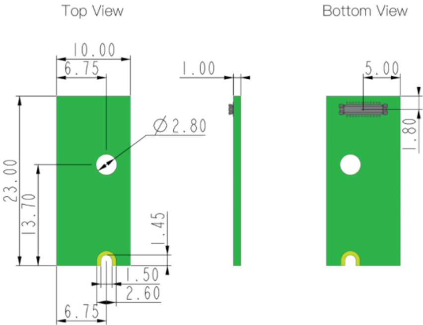
Figure 3: RAK12033 mechanical dimensions
