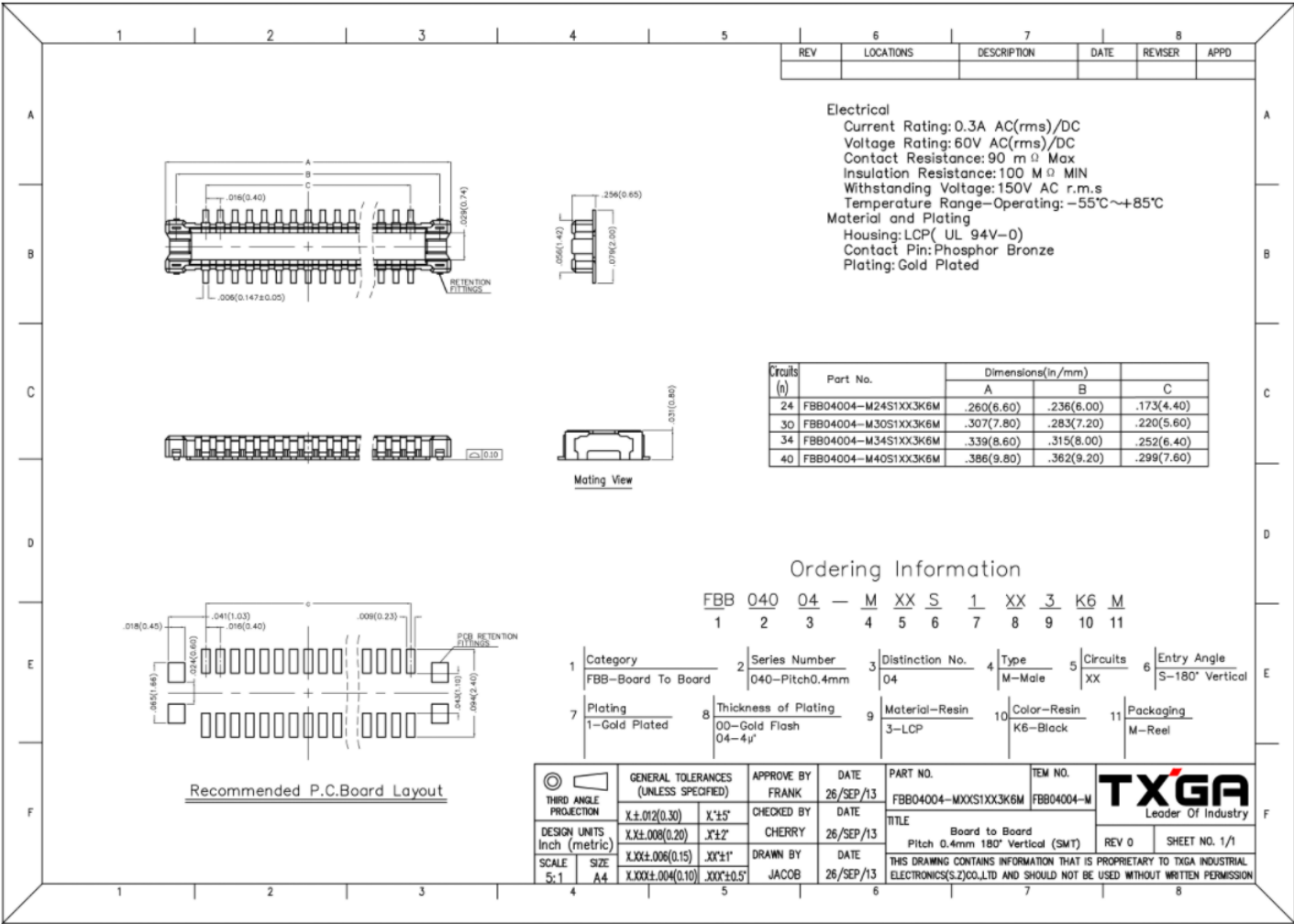
Figure 4: WisBlock Connector PCB footprint and recommendations
