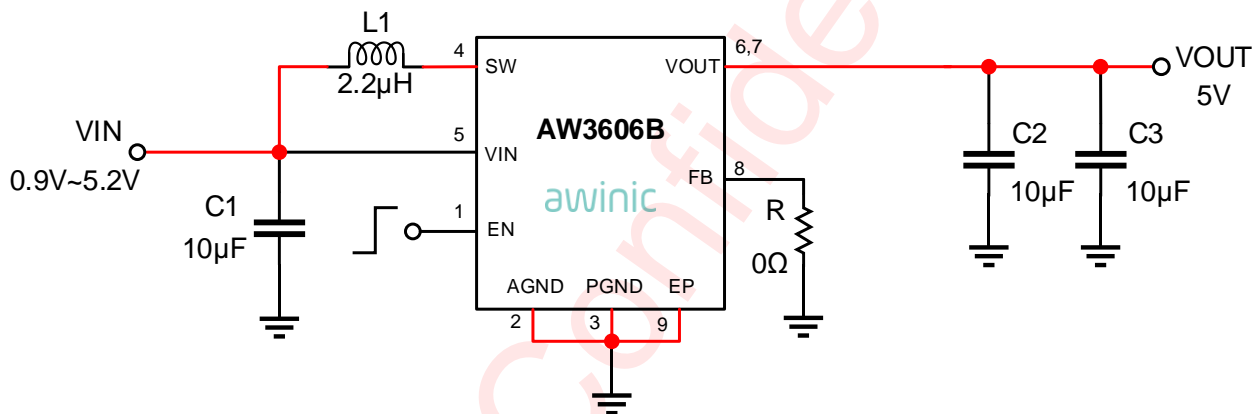
Typical Application Circuit of AW3606B
