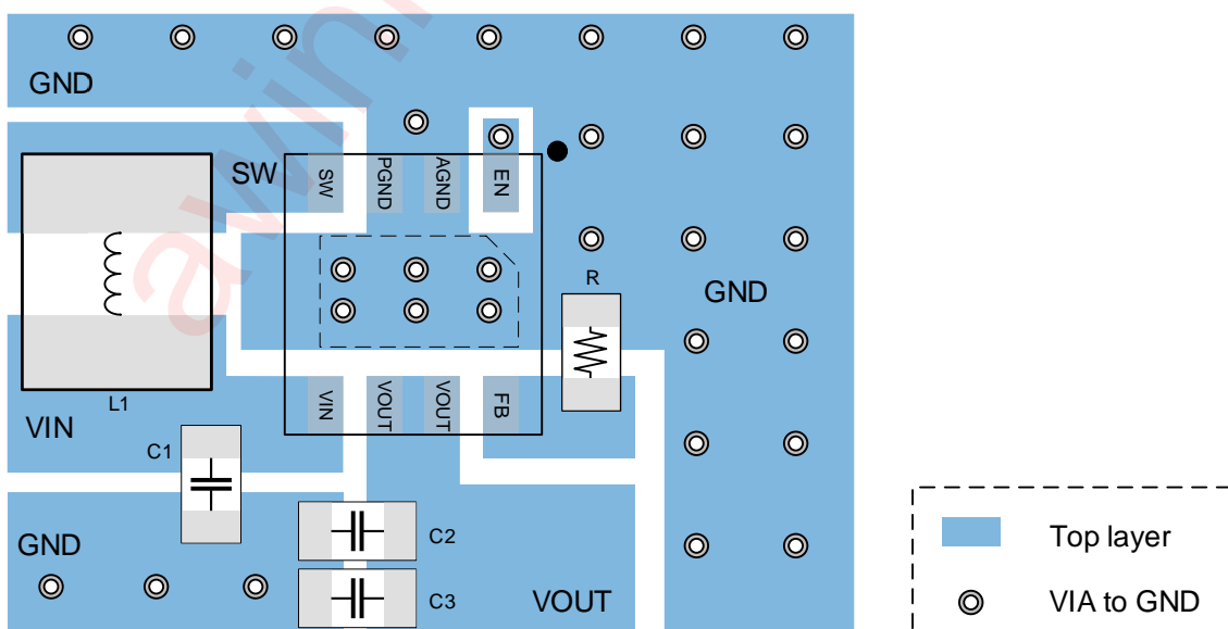
AW3606B Layout Recommendation
