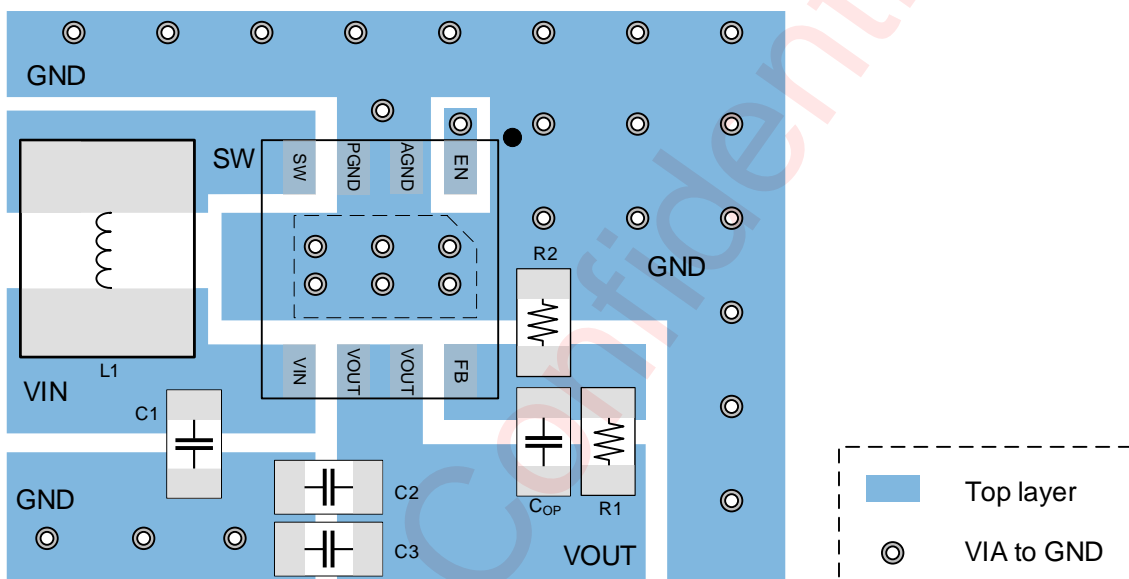
AW3606A Layout Recommendation
