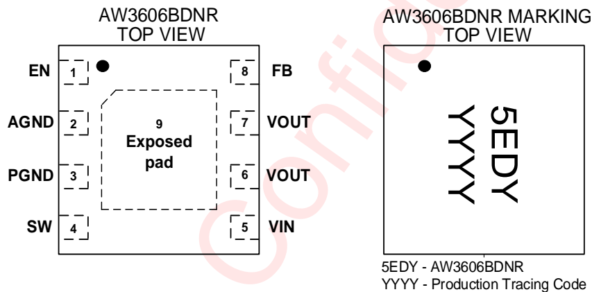
Pin Configuration and Top Mark of AW3606B
