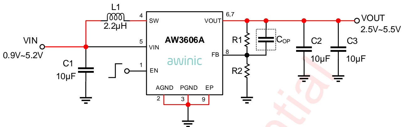
Typical Application Circuit of AW3606A
