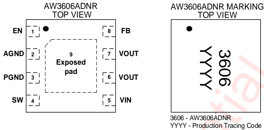
Pin Configuration and Top Mark of AW3606A
