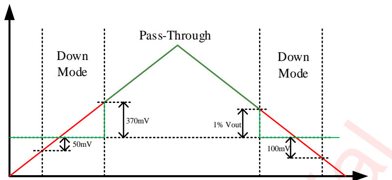
Down Mode and Pass-Through Mode
