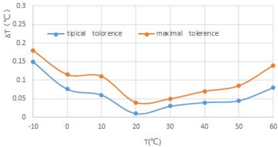
Figure 7-4 M601Z / M1601Z /M1820Z/ MTS01Z accuracy curve
