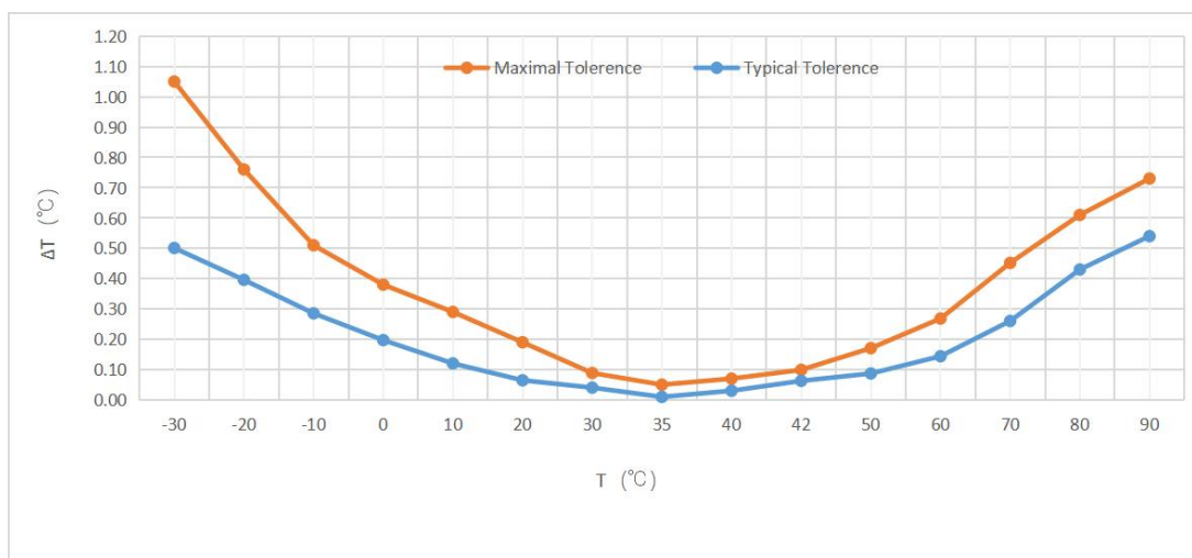
Figure 7 - 1 M601 / M1601 / MTS01 accuracy curve
