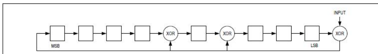
Figure 11.3 cyclic redundancy check generator
