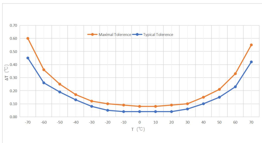
Figure 7-3 M601P / M1601P / M1820P/ MTS01P accuracy curve
