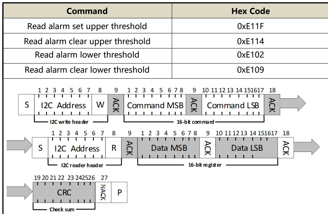
Fig. 12.14-1 Read alarm threshold command (Note: the white block is controlled by the microcontroller, and the sensor response is gray block.)
