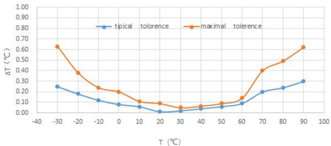
Figure 7-2 M601W / M1601W / M1820W/ MTS01W accuracy curve
