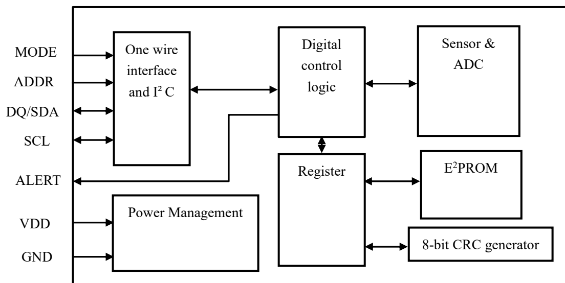
Figure 5 Diagram of digital thermometer
