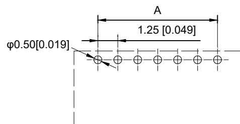
Recommended P.C.B Layout General Tolerance \pm 0.05
