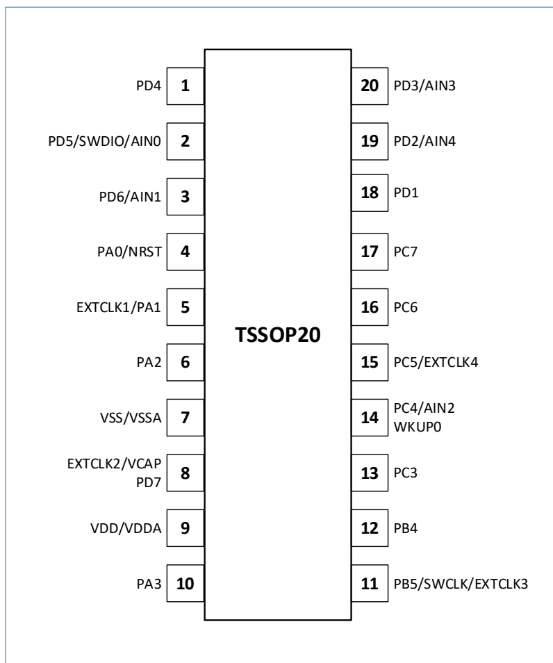
Figure 6-3 TSSOP20 pinout
