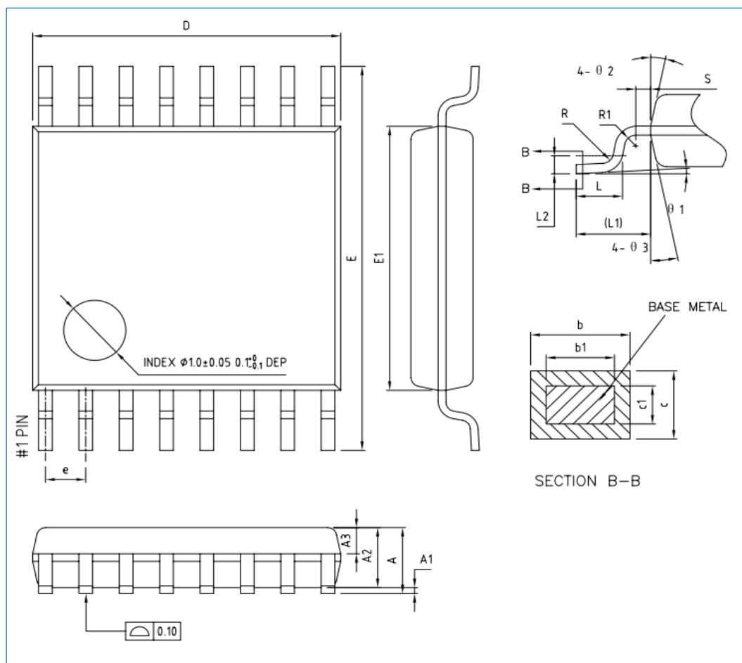
Figure 7-2 TSSOP16 package outline
