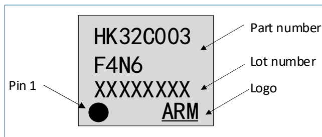
Figure 7-10 QFN20 HK32C003F4N6 marking example
