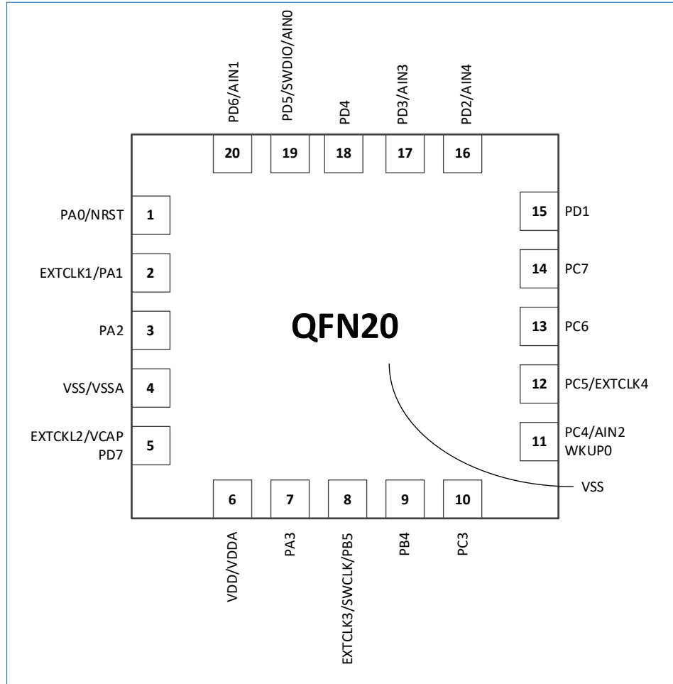
Figure 6-4 QFN20 pinout
