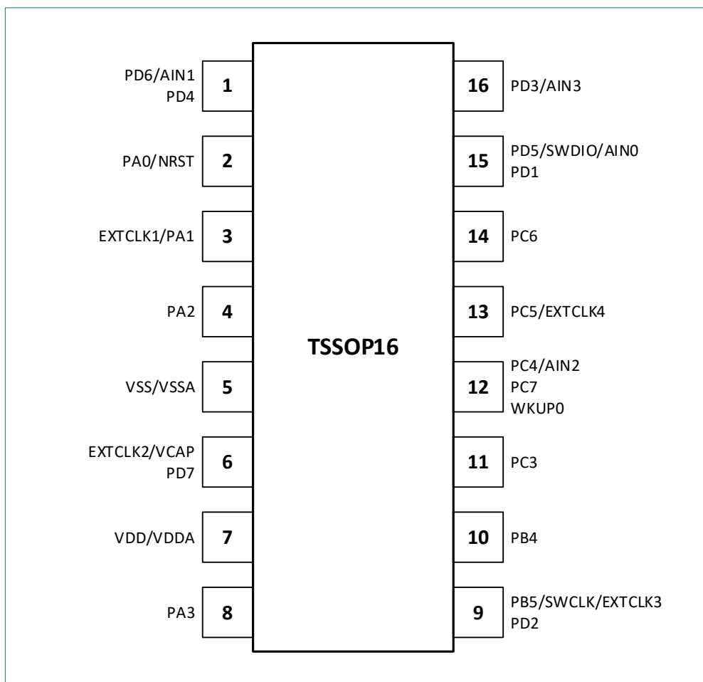
Figure 6-2 TSSOP16 pinout
