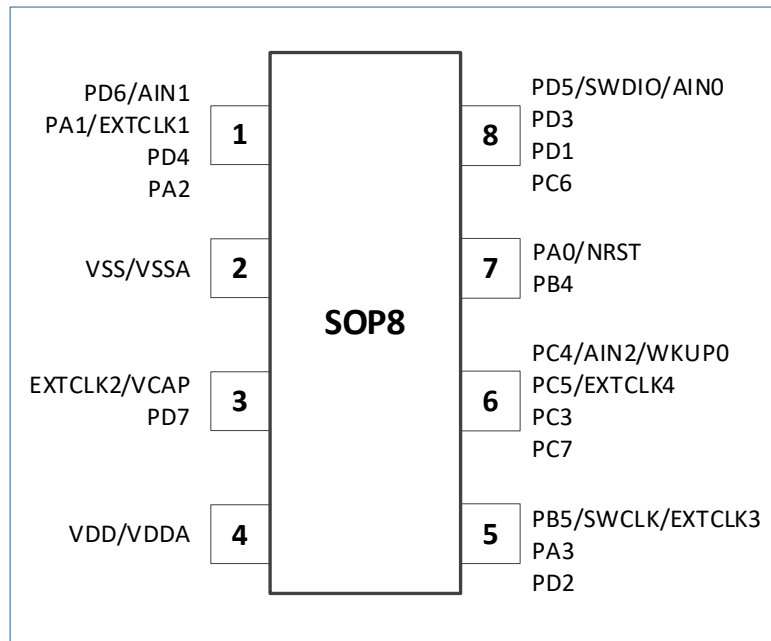
Figure 6-1 SOP8 pinout
