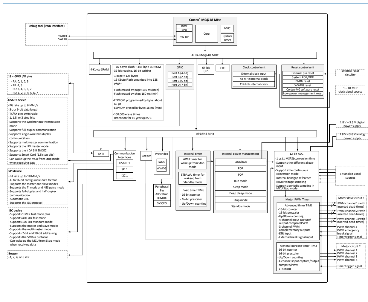
Figure 3-1 HK32C003F4U6 block diagram
