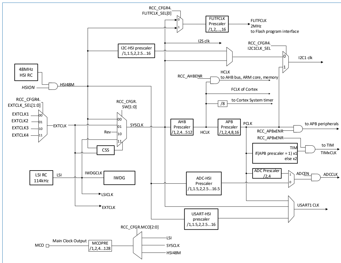
Figure 3-4 Clock tree
