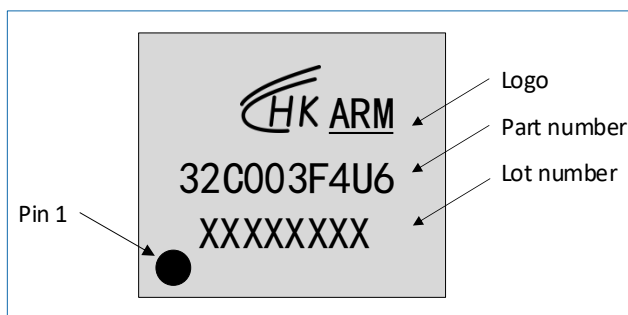
Figure 7-11 QFN20 HK32C003F4U6 marking example
