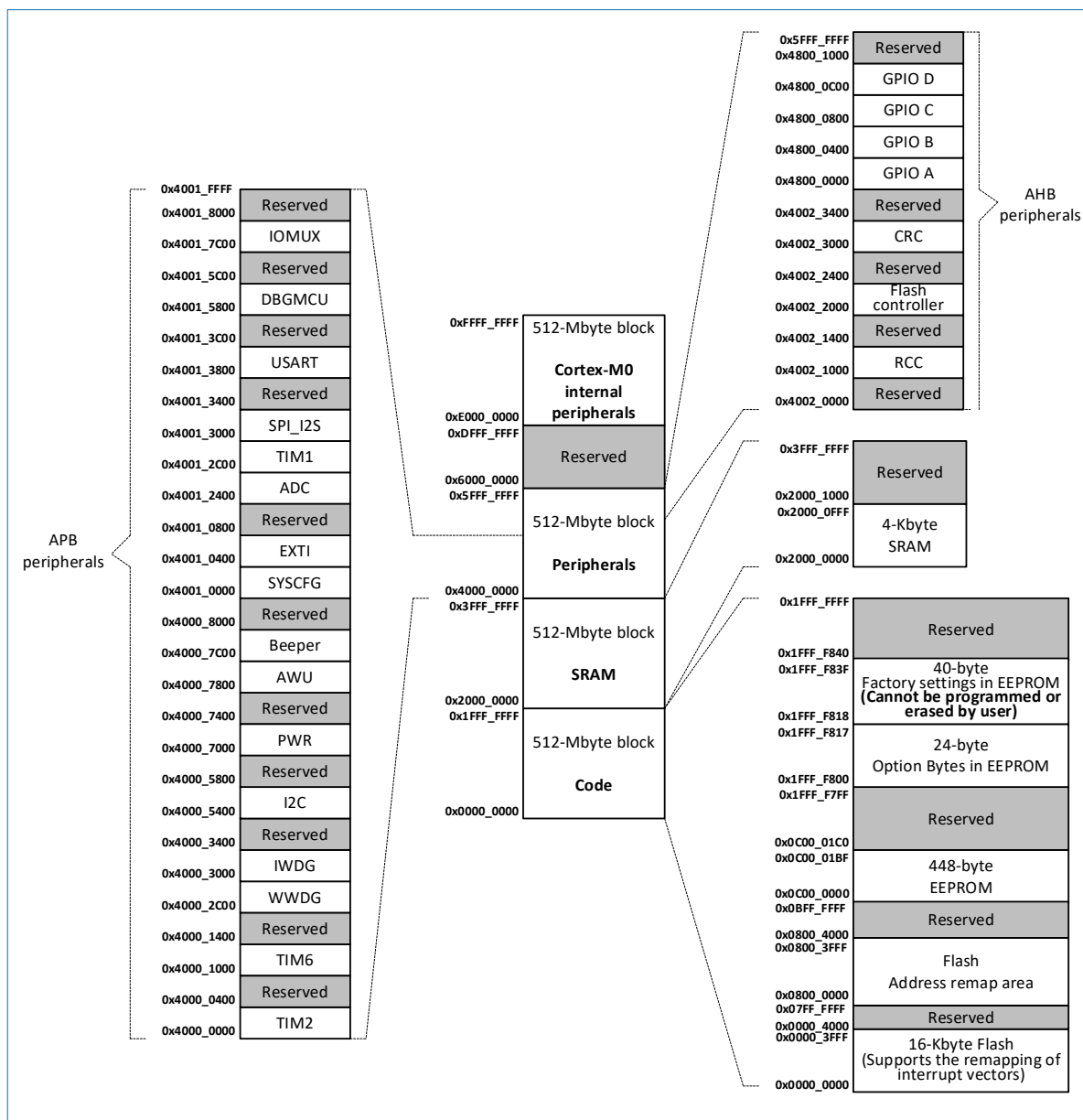
Figure 3-2 HK32C003 memory mapping
