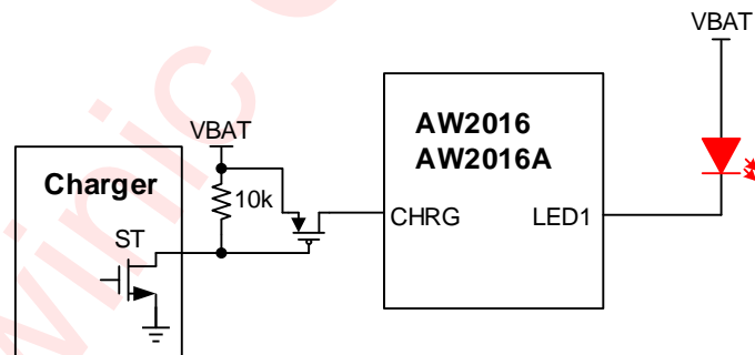
Figure 17 Real Charging Status Indication in Special Charger IC Application
