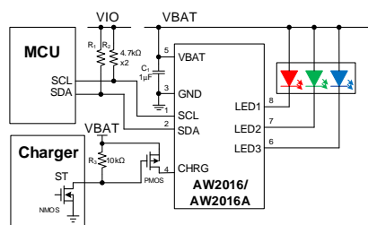
Charging Status Indication Application
