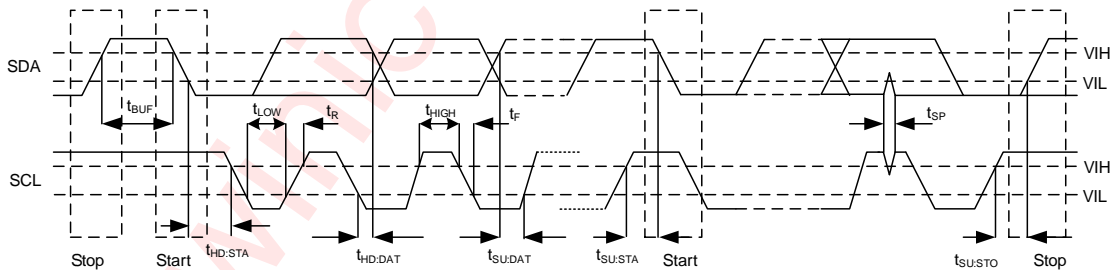
Figure 5 Timing of I 2 C Interface Signals
