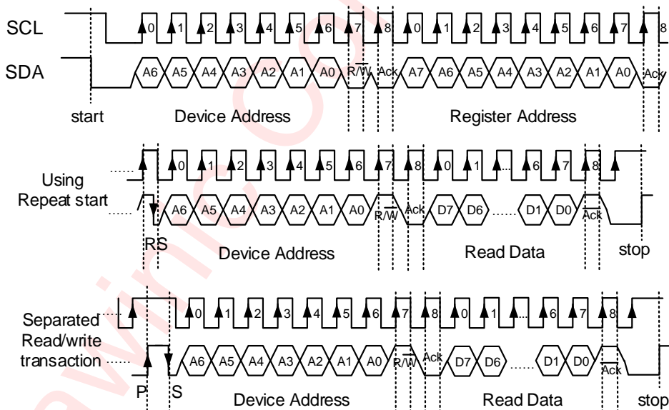
Figure 12 I 2 C Read Byte Cycle
