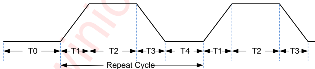
Figure 13 LED Breath Timing in Pattern Mode
