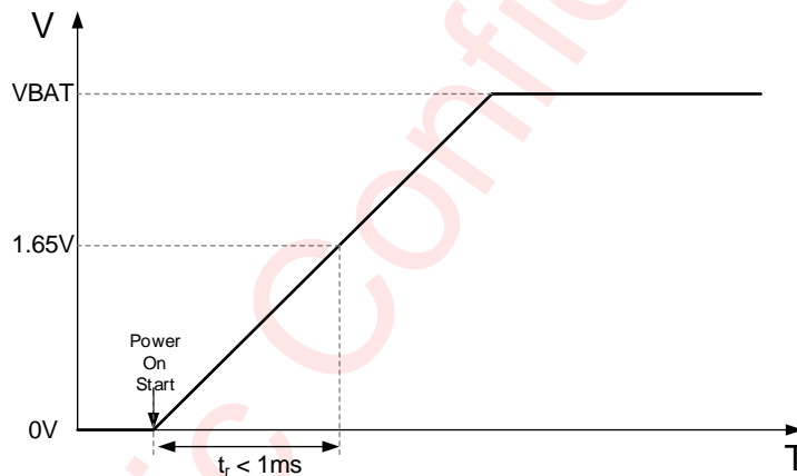
Figure 6 AW2016/AW2016A Power on Timing
