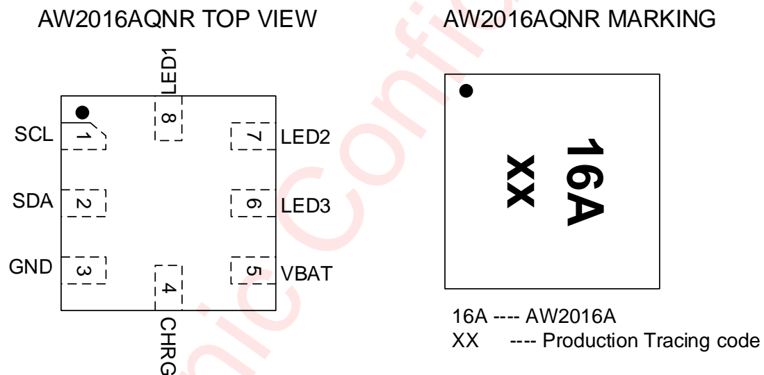
Figure 2 AW2016AQNR Pin Configuration and Top Marking
