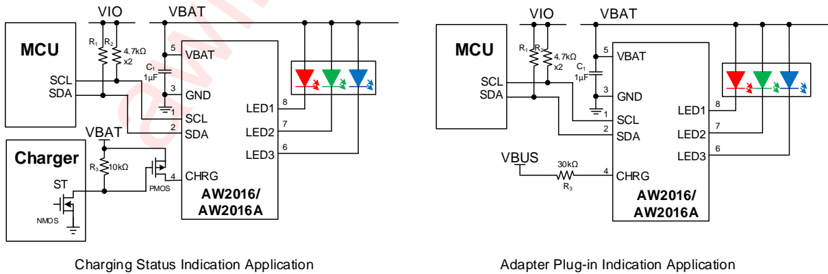
Figure 4 Typical Application Circuits
