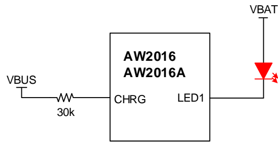
Figure 18 USB Power Insertion Status Indication in PMU-Controlled Charging Application
