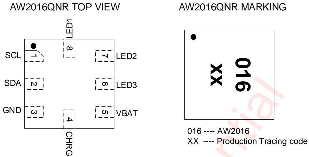
Figure 1 AW2016QNR Pin Configuration and Top Marking
