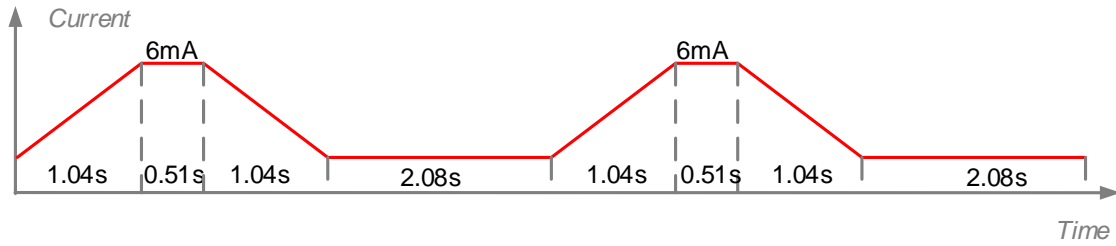
Figure 15 AW2016 Auto Charging Indication Pattern Parameter
