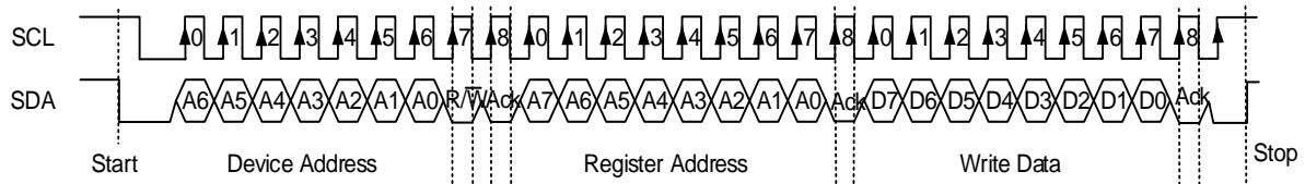
Figure 11 I 2 C Write Byte Cycle
