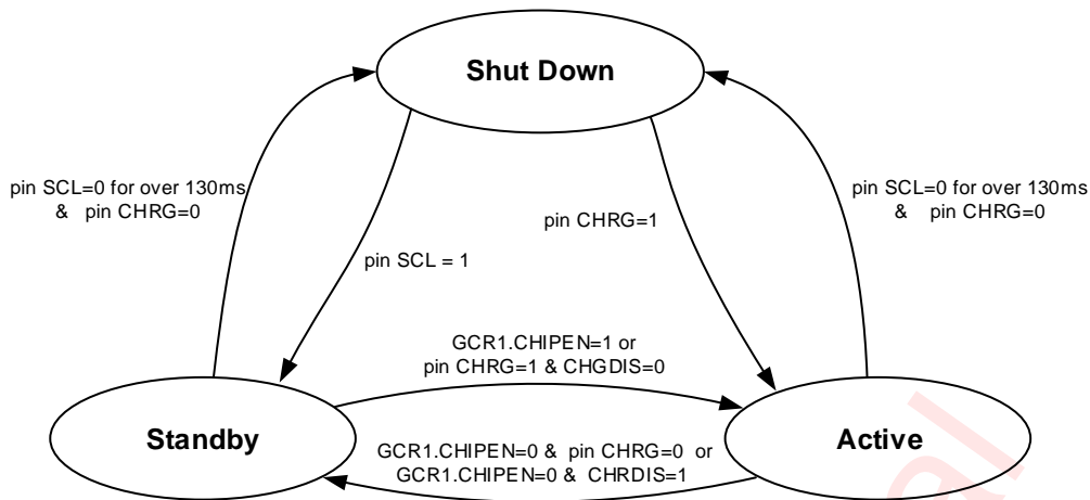
Figure 7 AW2016/AW2016A Operating Modes Transition
