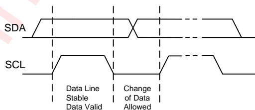
Figure 8 Data Validation Diagram
