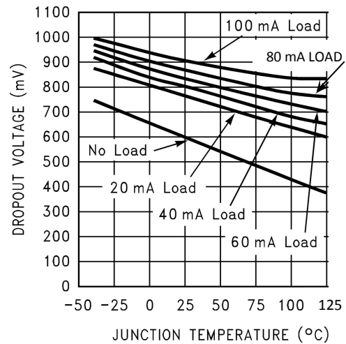
Figure 2. Dropout Voltage vs Junction Temperature
