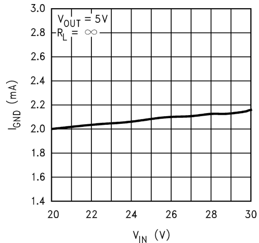
Figure 4. Ground Pin Current vs Input Voltage
