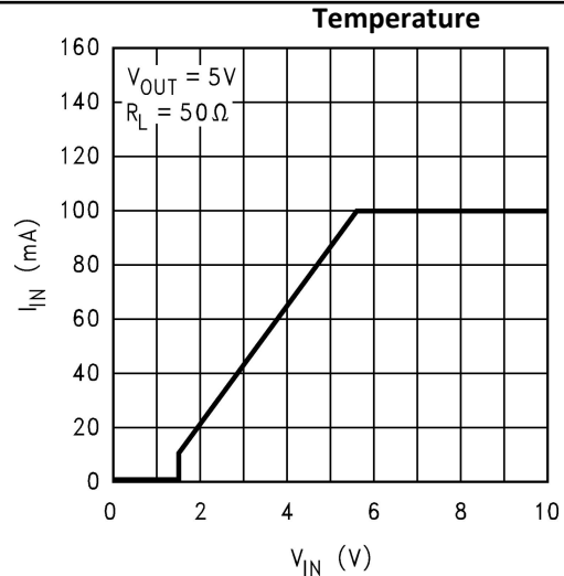
Figure 8. Input Current vs Input Voltage
