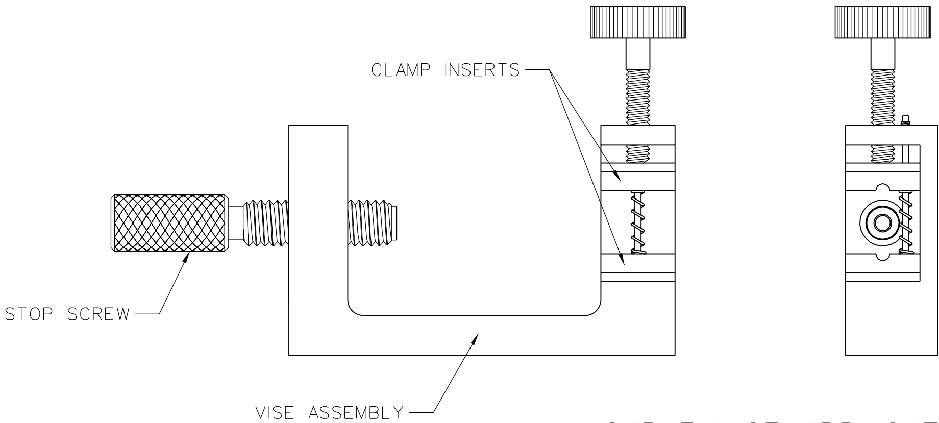
CABLE VISE APPLICATION 1.5:1 (FOR REFERENCE ONLY)
