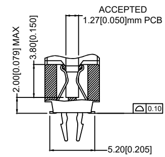
SECTION E-E SCALE 2:1
