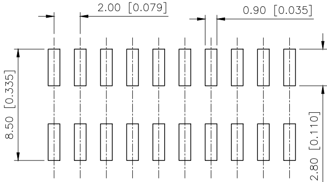
PCB LAYOUT
