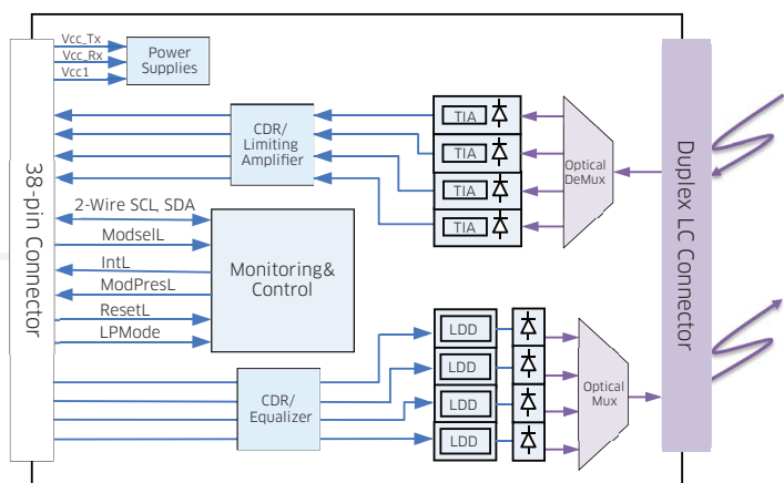
Figure 1. Lumentum QSFP28 CWDM4 Optical Transceiver functional block diagram
