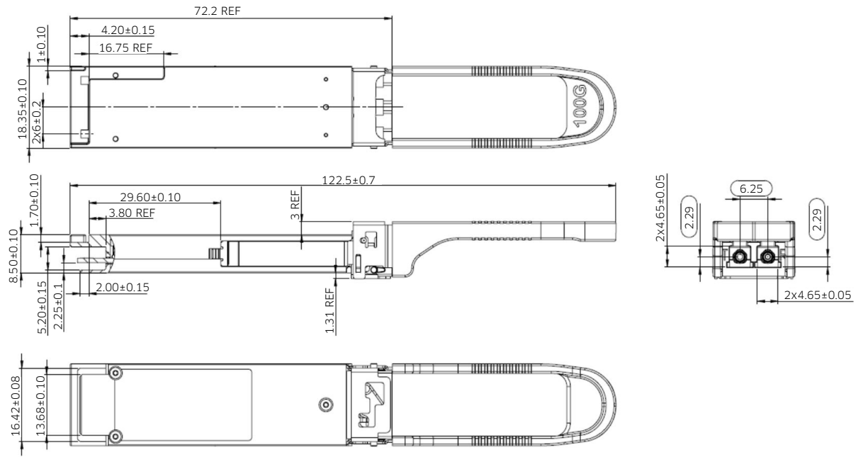
Module outline with pull tab
