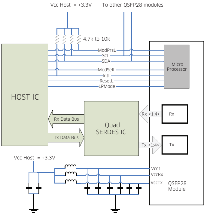
Figure 2. Typical application schematics for the Lumentum QSFP28 optical transceiver
