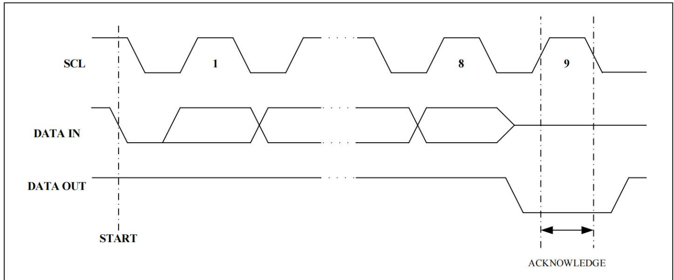
Figure 4. Output Acknowledge
