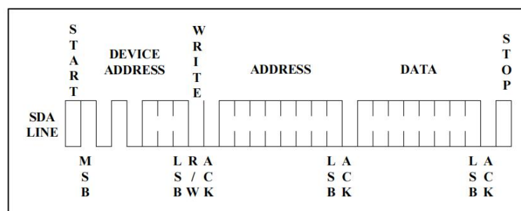
Figure 7. Byte Write
