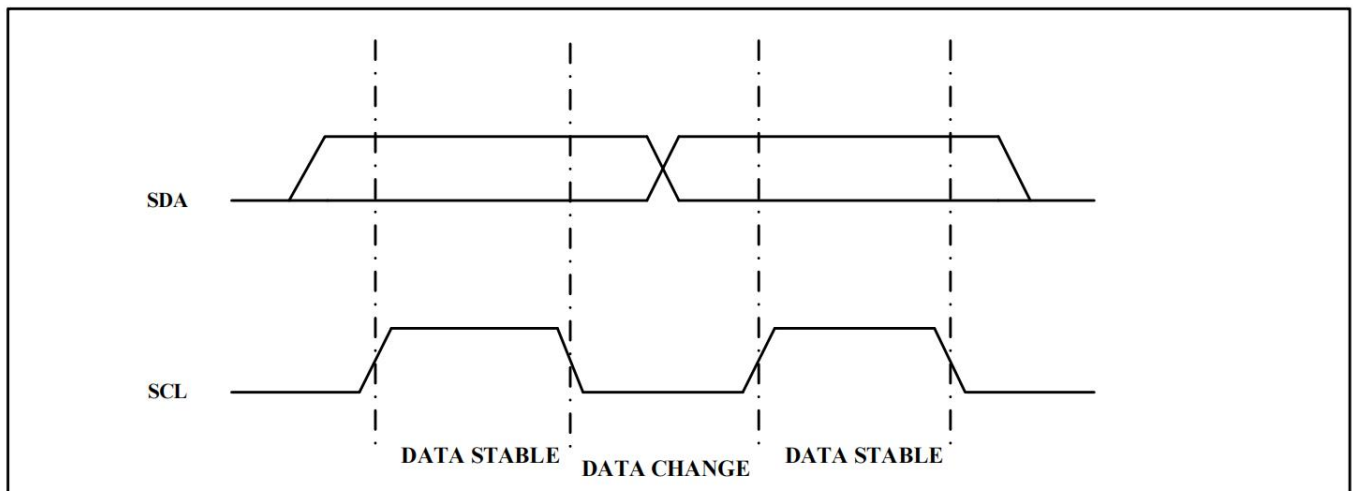
Figure 2. Data Validity
