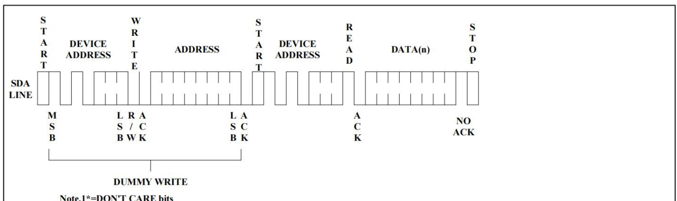
Figure 10. Random Read
