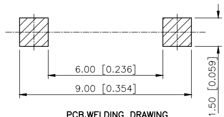
PCB.WELDING DRAWING
