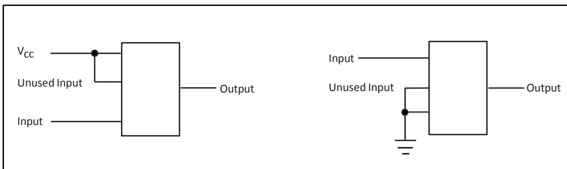
Figure 11-1. Layout Diagram
