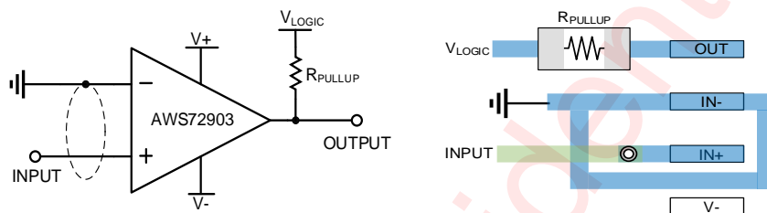
Figure 24 Non-inverting Comparator Application Schematic and Layout Example
