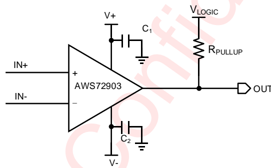
Figure 22 AWS72903 Schematic Example
