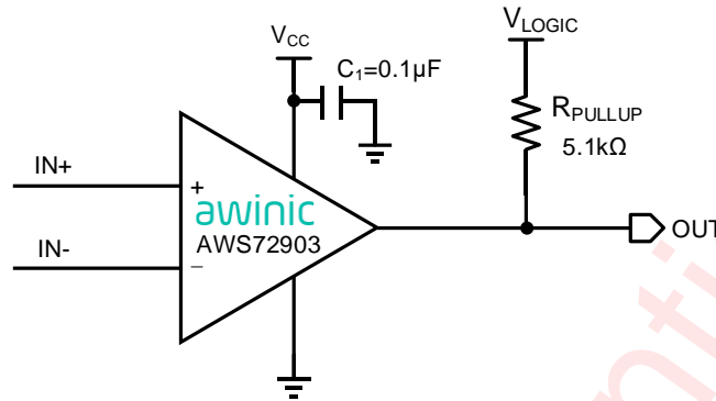
Figure 4 AWS72903 Application Circuit
