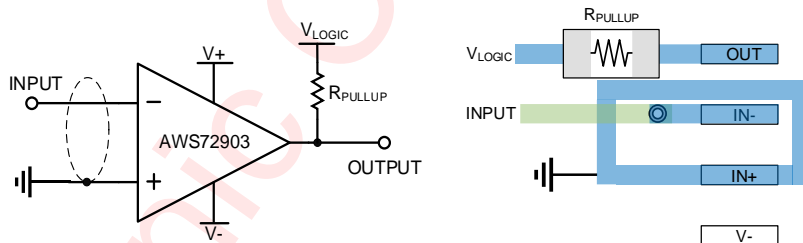
Figure 25 Inverting Comparator Application Schematic and Layout Example
