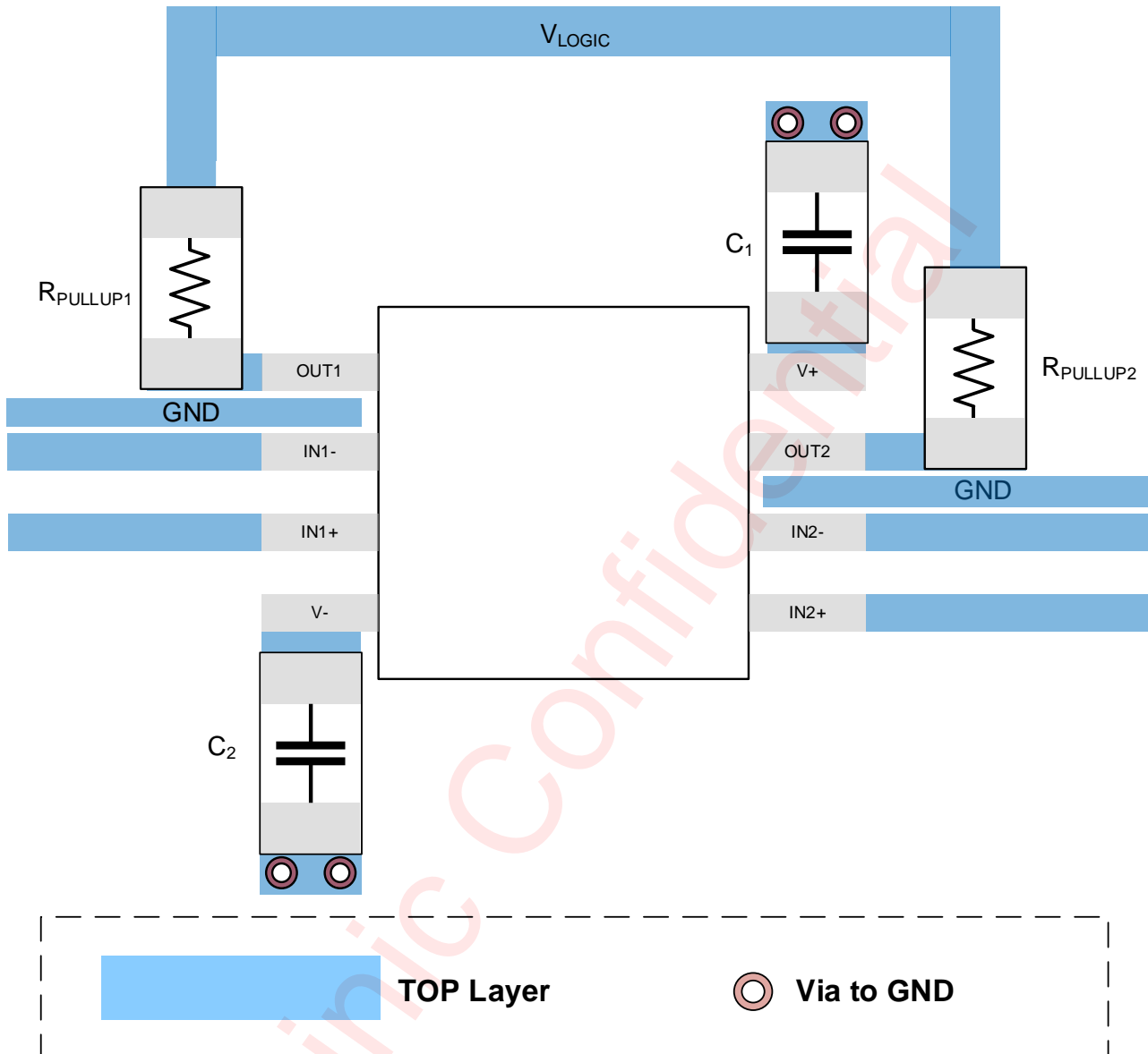
Figure 23 AWS72903 Layout Example
