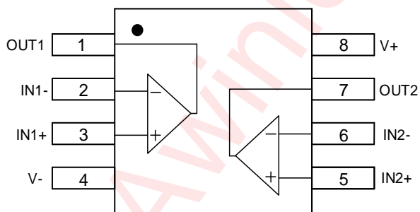
AWS72903MPR (Top view)
