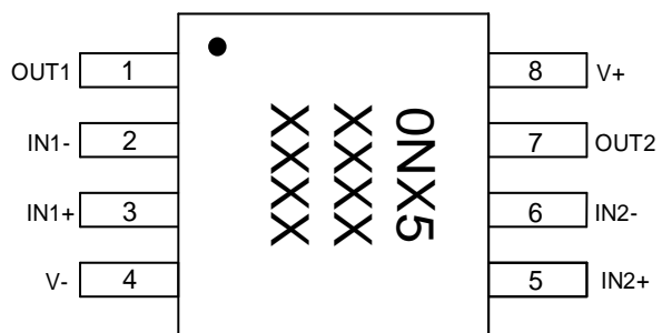
AWS72903MPR Marking (Top view)
