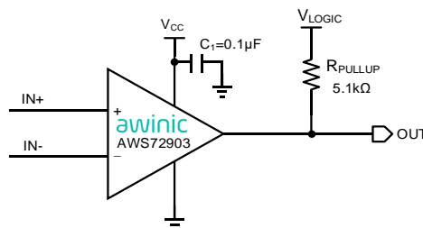
Figure 1 Typical Application of AWS72903
