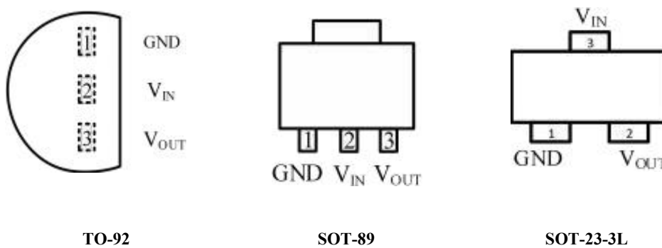
Figure 2.HT75XX Pin
