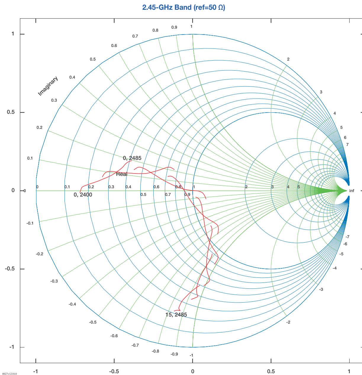
Figure 2-2 • Combined Port Impedance (2400 to 2485GHz)
