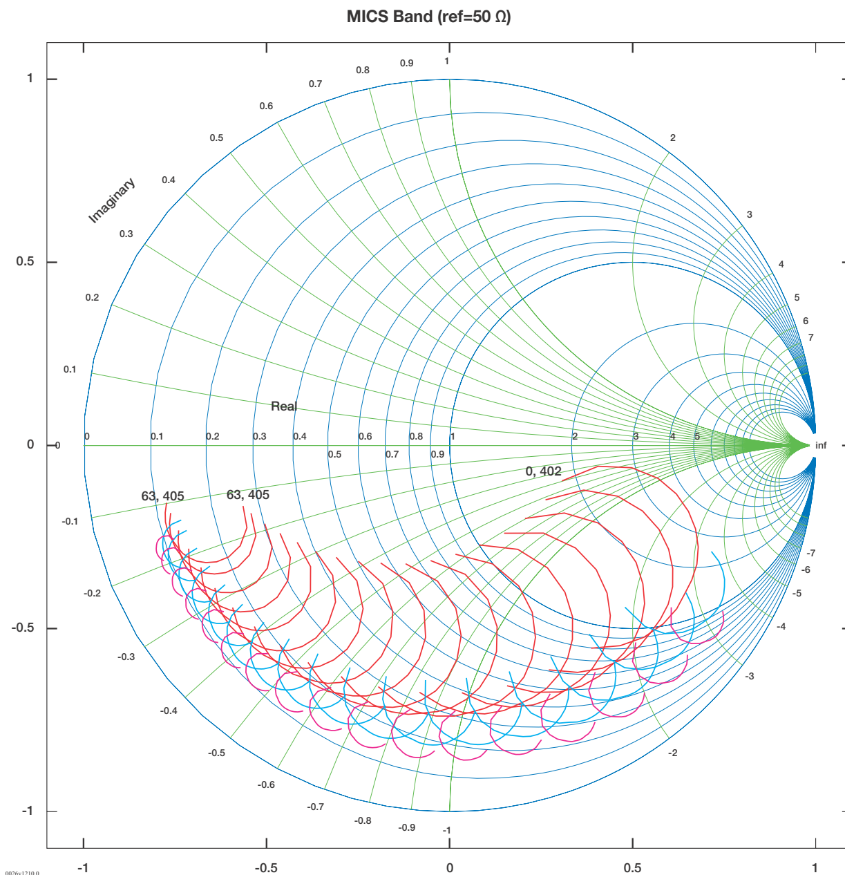
Figure 2-1 • Combined Port Impedance (402 to 405MHz)
