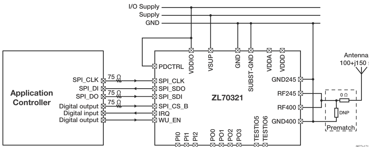
Figure 5-1 • Typical Application Example
