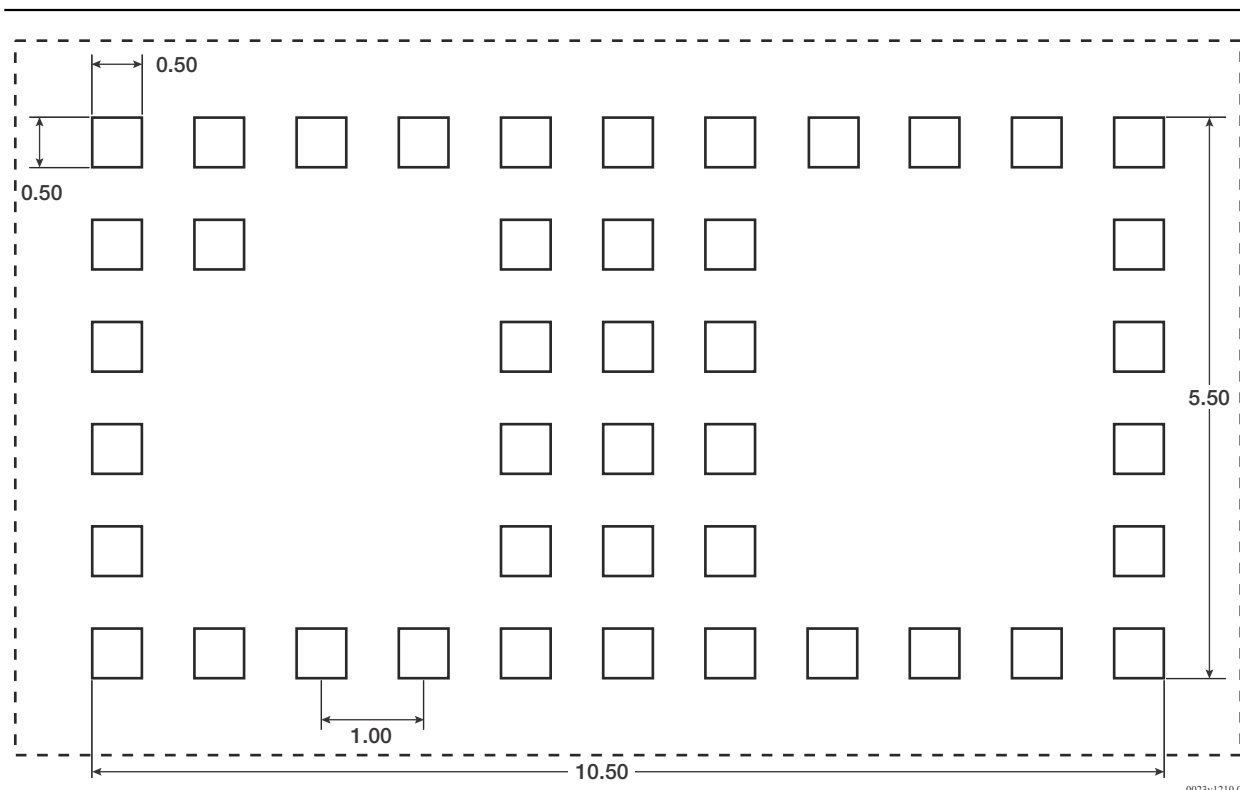
Figure 4-3 • Recommended PCB Layout
