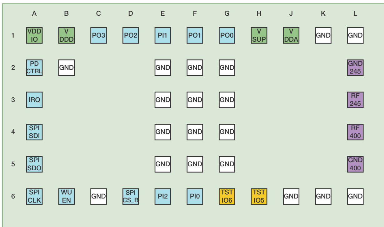
Figure 4-2 • ZL70321 Pad Configuration
