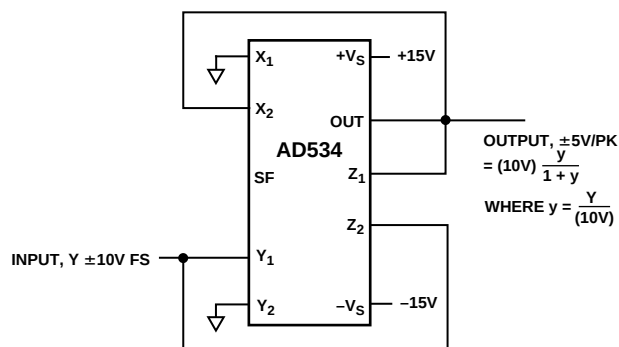
Figure 13. Bridge-Linearization Function
