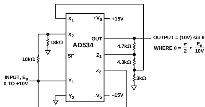
Figure 10. Sine-Function Generator
