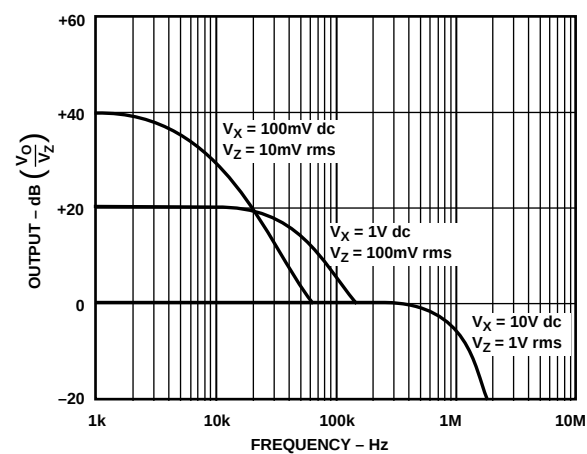
Figure 23. Frequency Response vs. Divider Denominator Input Voltage
