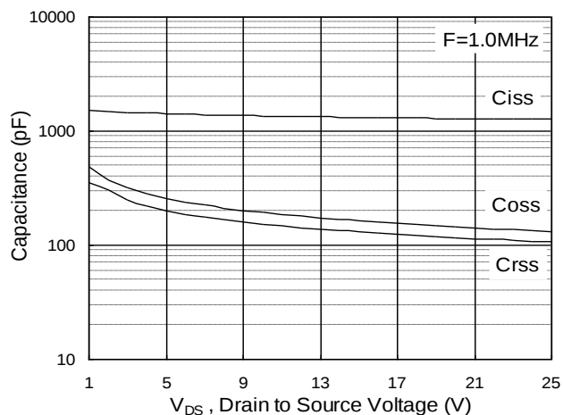
Fig.7 Capacitance
