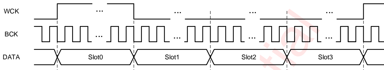
Figure 11 TDM Timing
