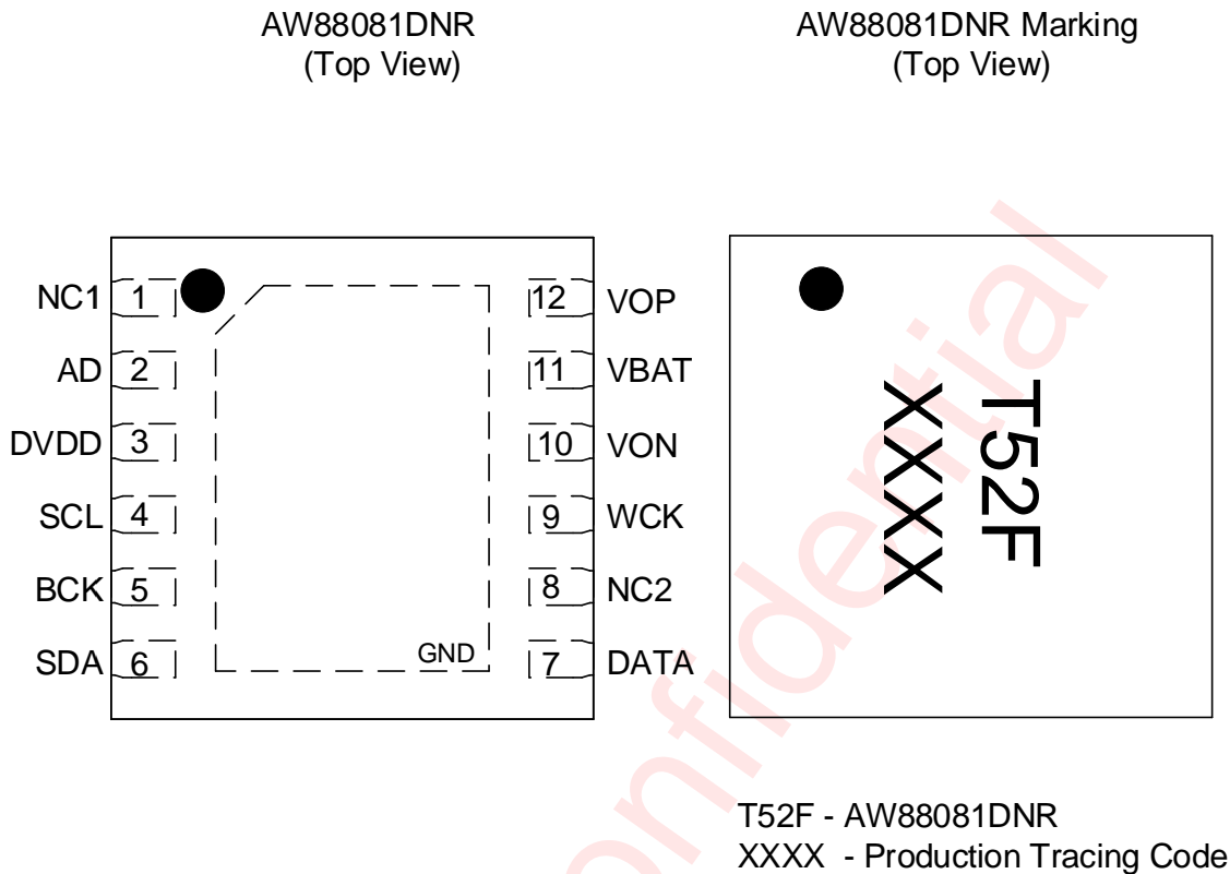
Figure 1 AW88081DNR pin diagram top view and device marking
