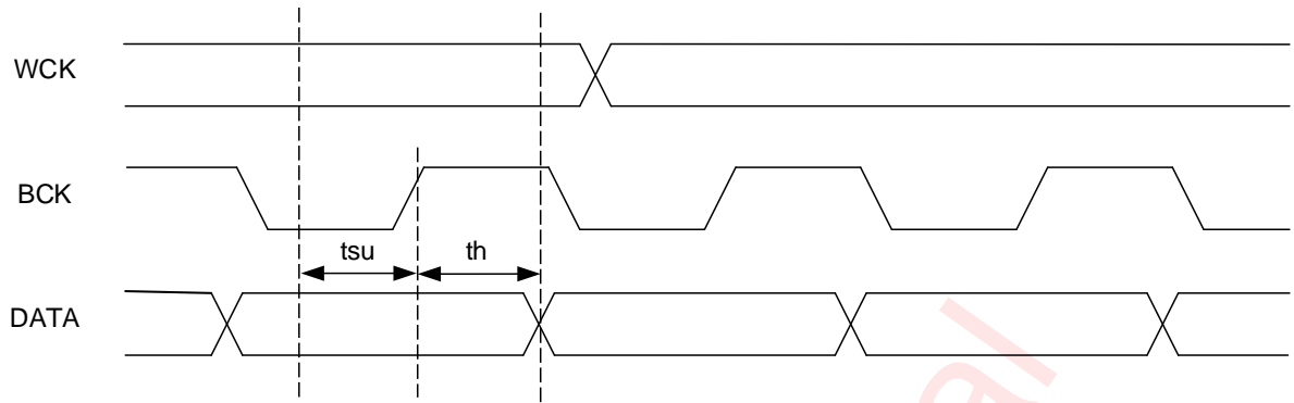
Figure 4 I 2 S Digital Audio Interface Timing
