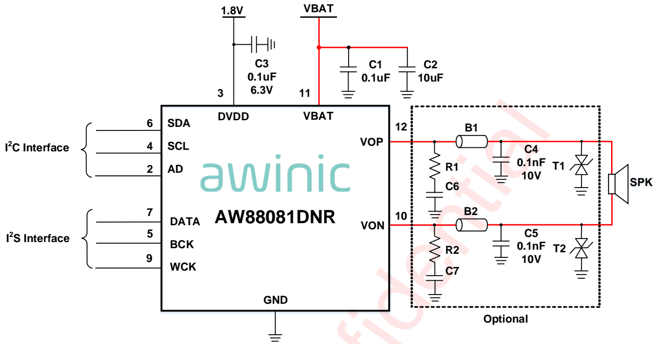
Figure 3 AW88081DNR Application Circuit
