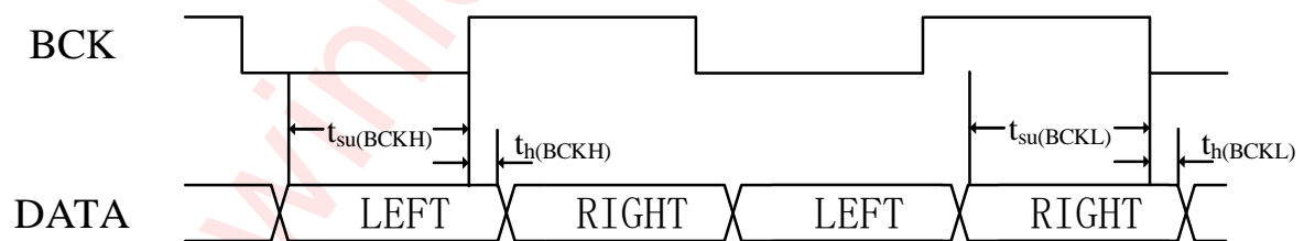
Figure 5 PDM Digital Audio Interface Timing
