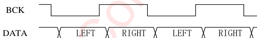
Figure 12 Digital stereo PDM Timing
