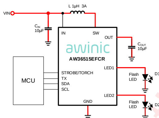
AW36515E Application Circuit
