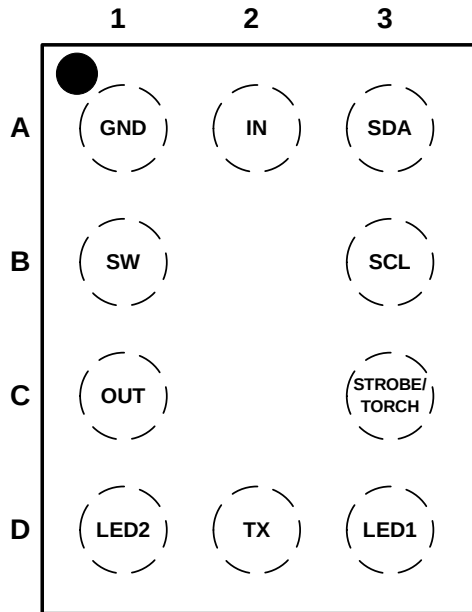
AW36515EFCR Pin Configuration (Top View)
