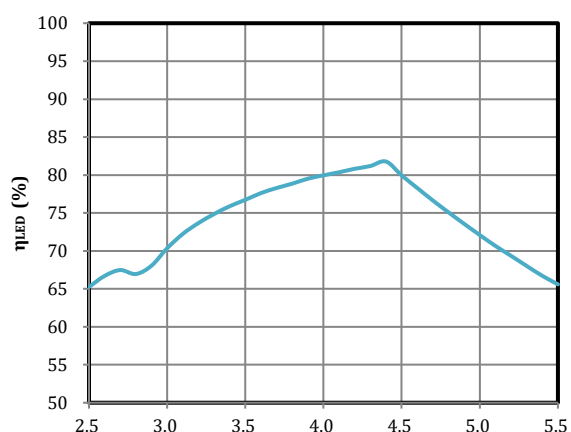
LED1/2 Efficiency vs Input Voltage
