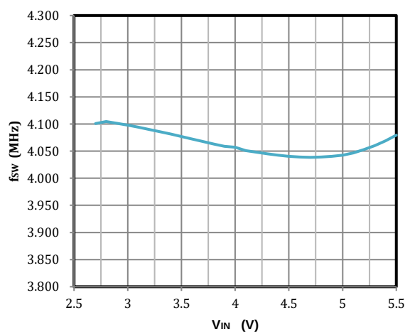
4-MHz Frequency vs Input Voltage
