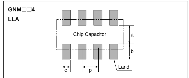
Part Number Dimensions (mm) L W a b c p GNM0M2 0.9 0.6 0.12 to 0.20* 0.35 to 0.40* 0.3 0.45 GNM1M2 1.37 1.0 0.4 to 0.5 0.35 to 0.45 0.3 to 0.35 0.64 GNM212 2.0 1.25 0.6 to 0.7 0.5 to 0.7 0.4 to 0.5 1.0 GNM214 2.0 1.25 0.6 to 0.7 0.5 to 0.7 0.25 to 0.35 0.5 GNM314 3.2 1.6 0.8 to 1.0 0.7 to 0.9 0.3 to 0.4 0.8 LLA18 1.6 0.8 0.3 to 0.4 0.25 to 0.35 0.15 to 0.25 0.4 LLA21 2.0 1.25 0.5 to 0.7 0.35 to 0.6 0.2 to 0.3 0.5 LLA31 3.2 1.6 0.7 to 0.9 0.4 to 0.7 0.3 to 0.4 0.8
