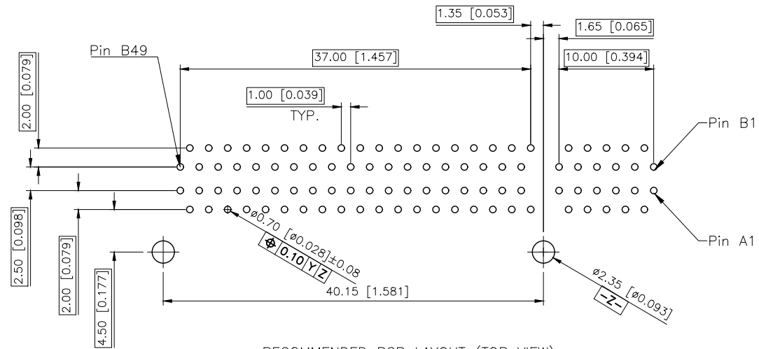
RECOMMENDED PCB LAYOUT (TOP VIEW) FOR 98P TOLERANCE: \pm 0.05 DATUM Y IS THE PCB SOLDER SURFACE
