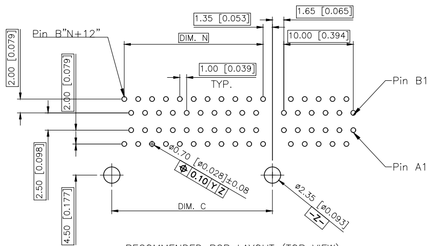
RECOMMENDED PCB LAYOUT (TOP VIEW) FOR 36P, 64P, 164P TOLERANCE: \pm 0.05 DATUM Y IS THE PCB SOLDER SURFACE
