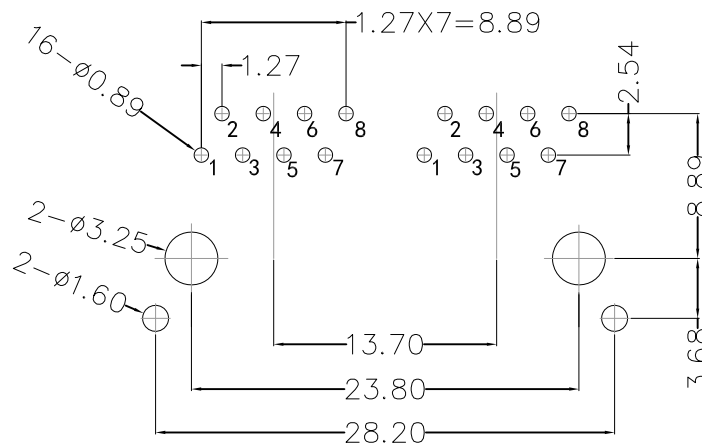
RECOMMENDED PCB LAYOUT VIEWED FROM COMPONENT SIDE
