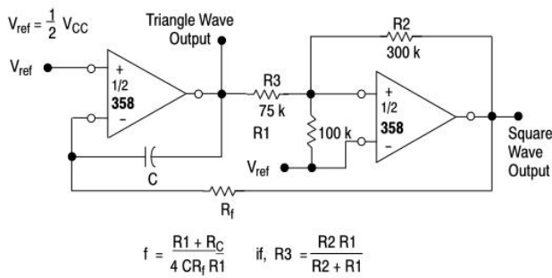
Figure 15. Function Generator
