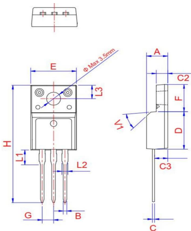
TO-220F
