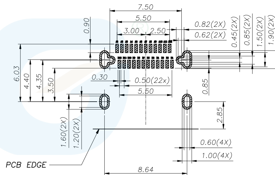
RECOMMENDED PCB LAYOUT(TOP VIEW) THICKNESS 1.20MM;DEFAULT TOLERANCE:±0.05
