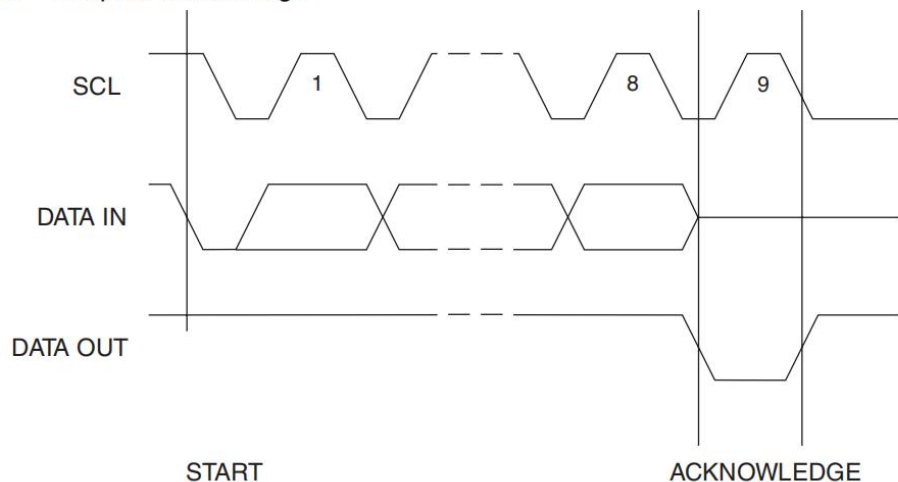
Figure 6-6. Output Acknowledge
