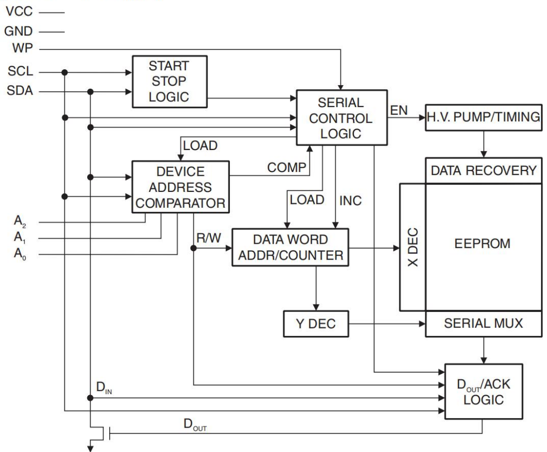
Figure 3-1. Block Diagram
