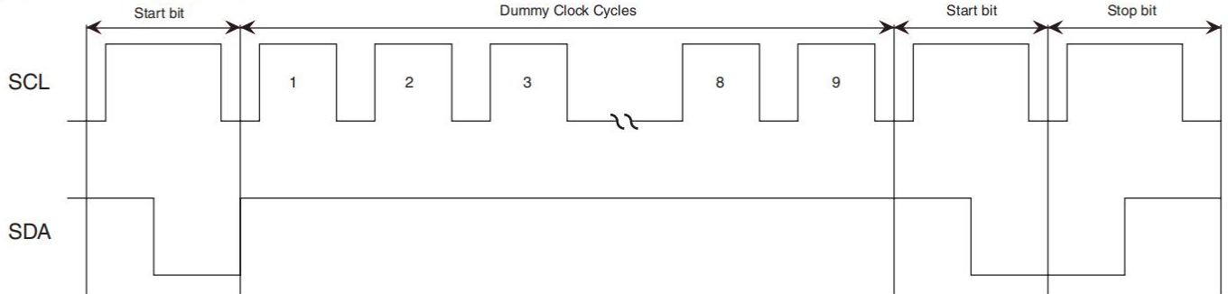
Figure 6-3. Software Reset
