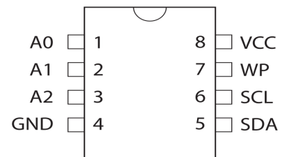
8-lead TSSOP
