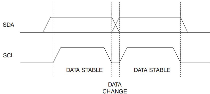
Figure 6-1. Data Validity
