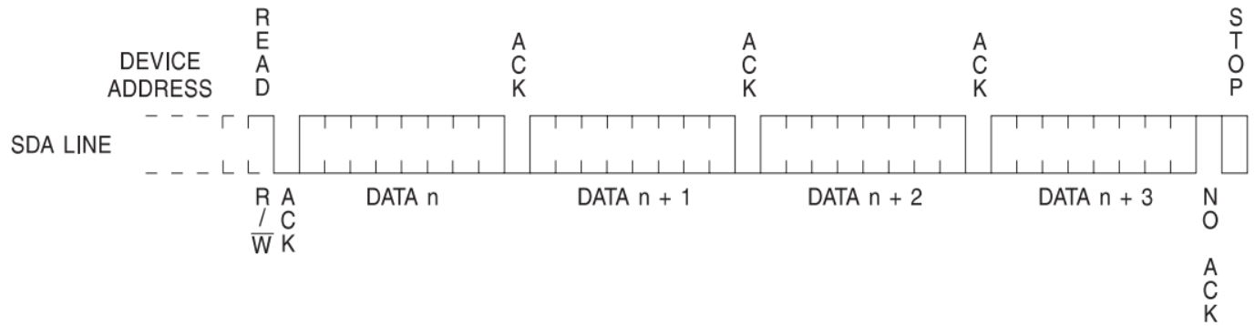
Figure 9-3. Sequential Read
