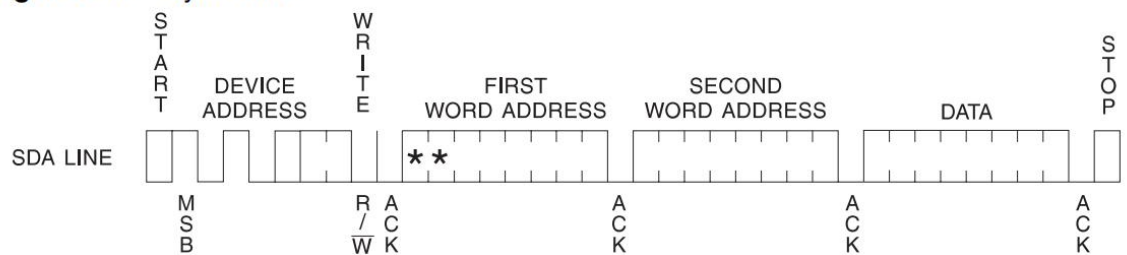
Figure 8-1. Byte Write
