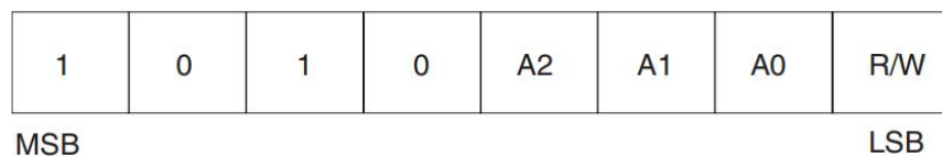
Figure 7-1. Device Address
