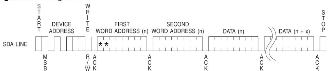
Figure 8-2. Page Write
