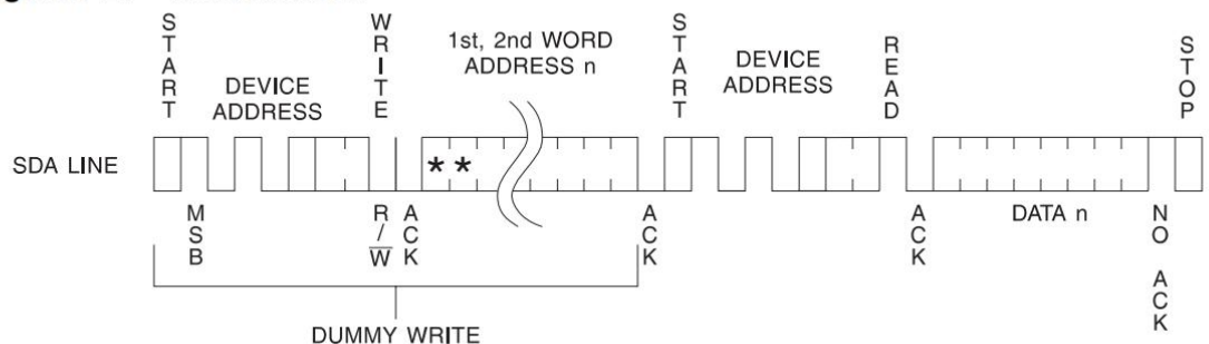
Figure 9-2. Random Read
