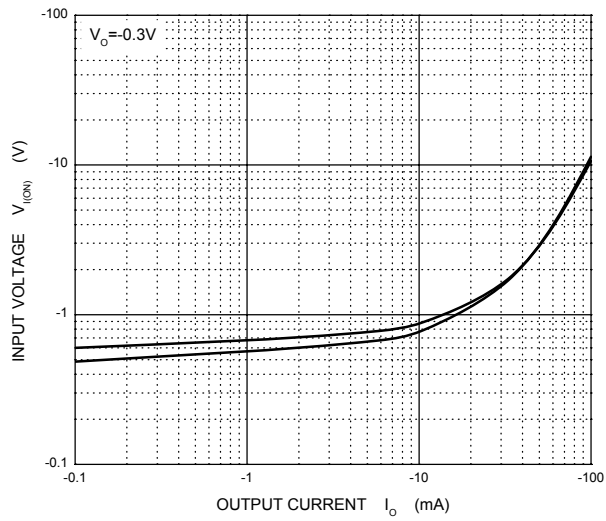
ON Characteristics
