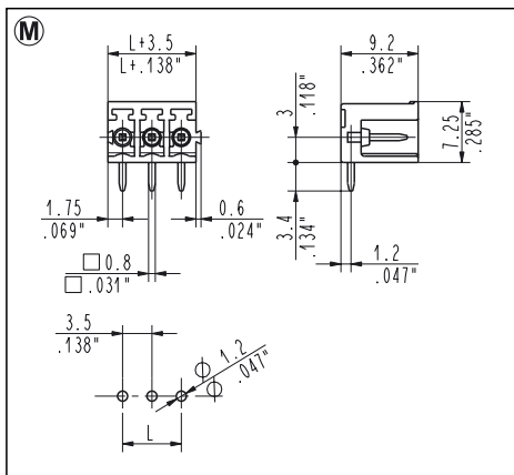
CTM_9M8 90°, Modular-Side Stackable Male 3.5 mm / .138" Pitch Weight per pole: 0.21 g
