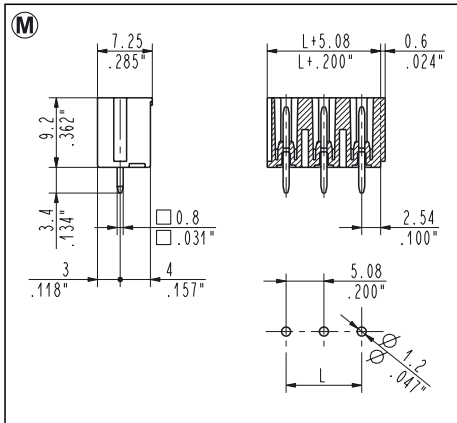
CTM_0M5 Straight, Modular-Side Stackable Male 5.08 mm / .200" Pitch Weight per pole: 0.29 g
