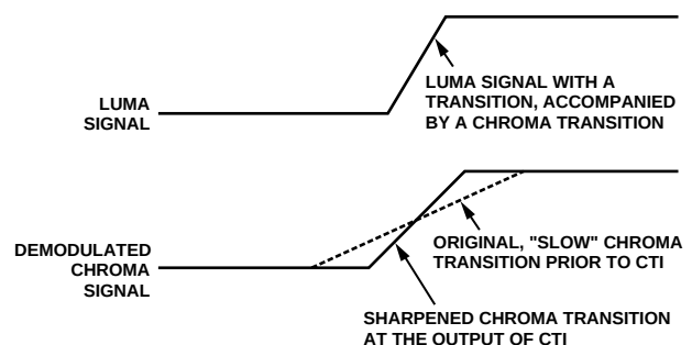
Figure 18. CTI Luma/Chroma Transition
