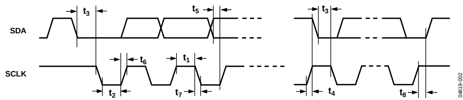
Figure 2. I²C Timing
