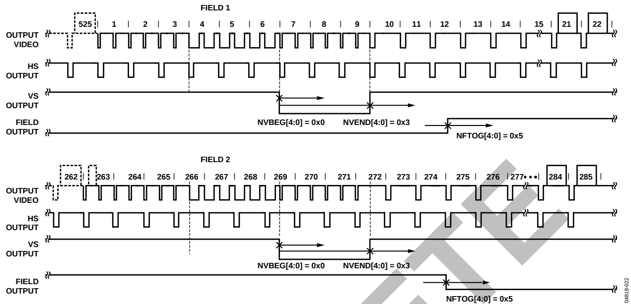
Figure 22. NTSC Typical VSync/Field Positions Using Register Writes in Table 109
