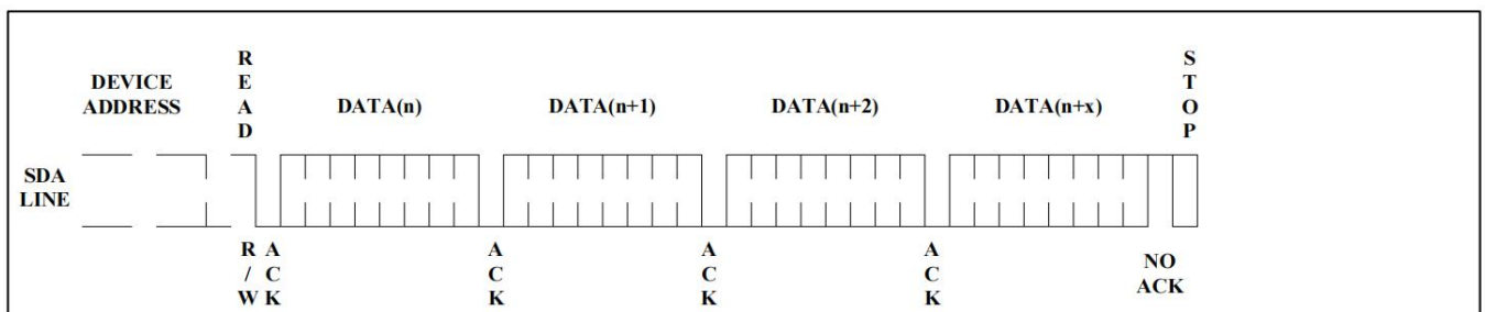
Figure 10. Sequential Read
