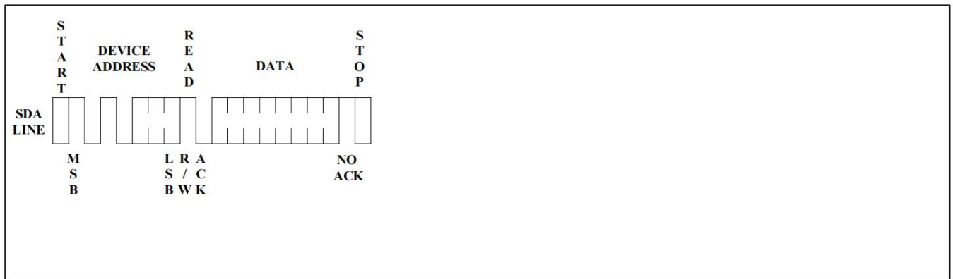
Figure 9. Random Read
