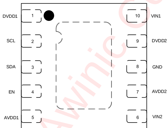
AW37004DNR (Top View)
