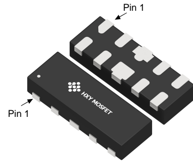
DFN2510-10L (DFN2510-10)
