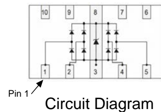
DFN2510-10L (DFN2510-10)
