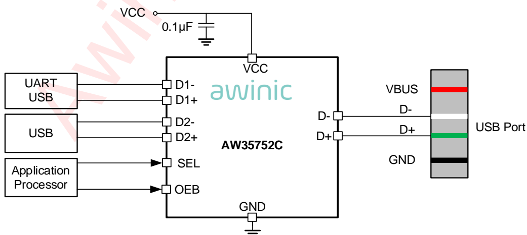
Figure 1 Typical Application Circuit of AW35752C
