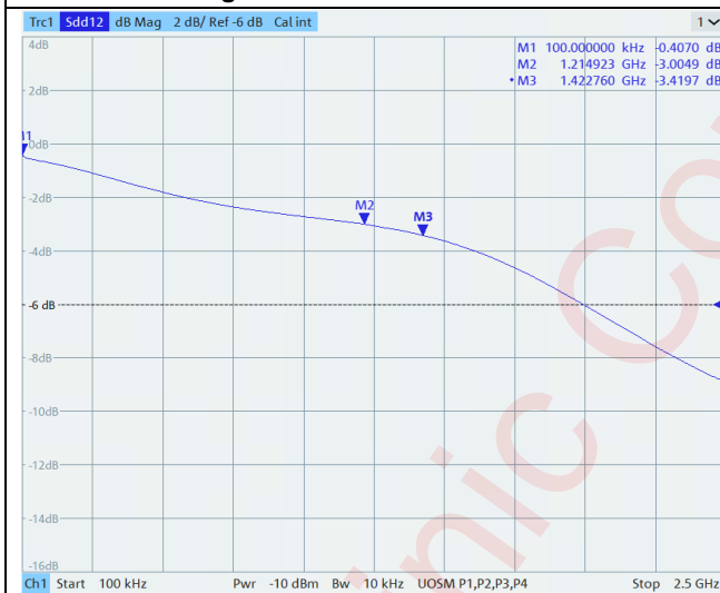
Figure 13 BW of D± to D1±
