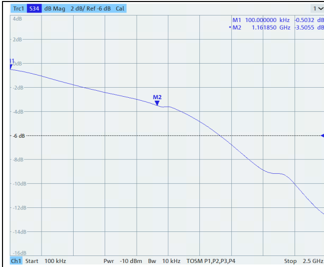
Figure 11 BW of D+ to D2+
