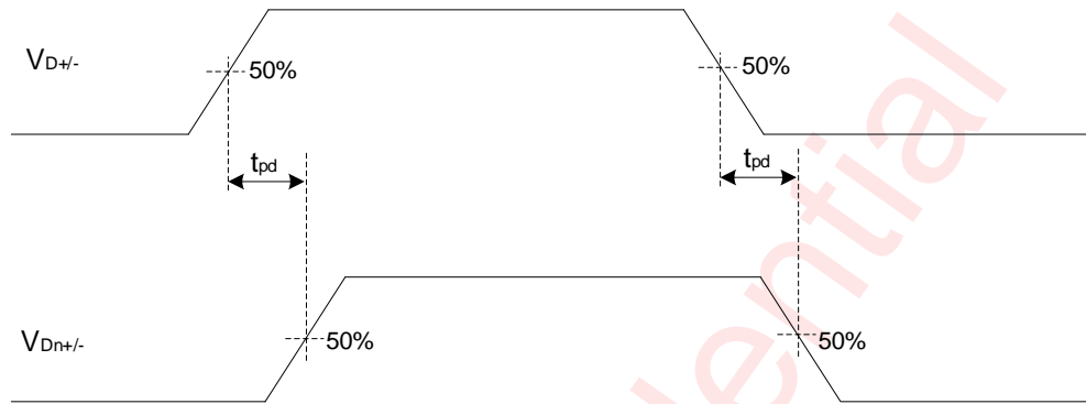
Figure 19 Propagation delay
