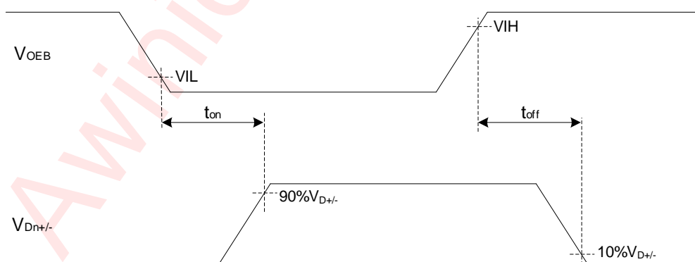
Figure 18 Device Turn On Time
