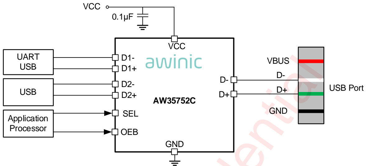
Figure 4 Typical Application Circuit of AW35752C
