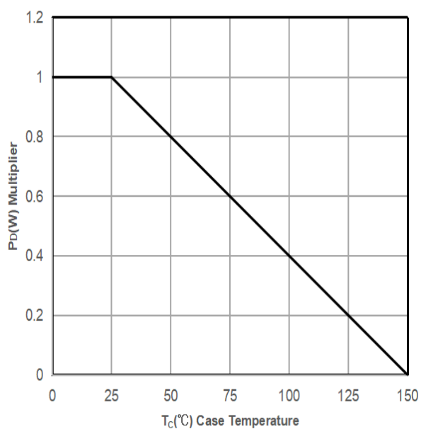
Power Capability
