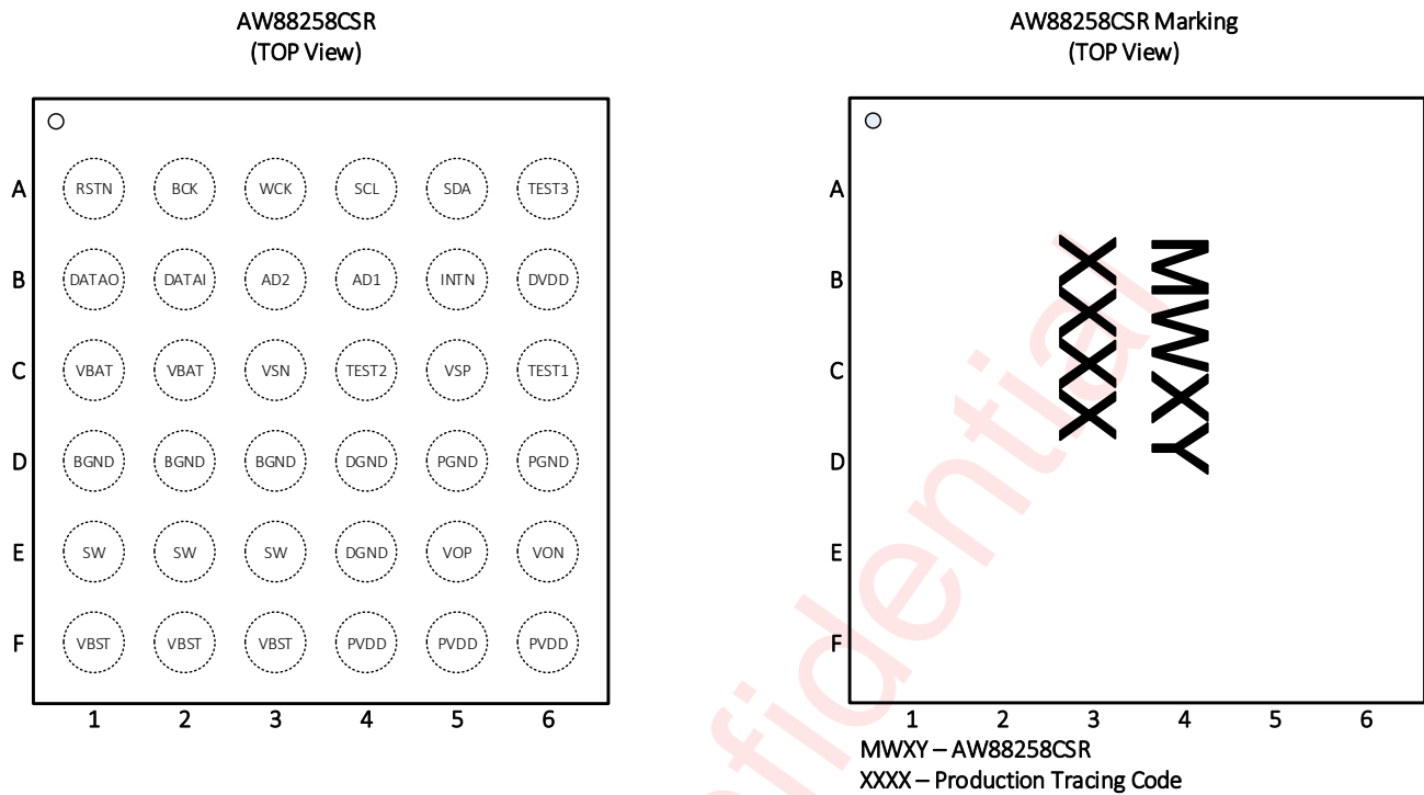
Figure 1 AW88258CSR pin diagram top view and device marking
