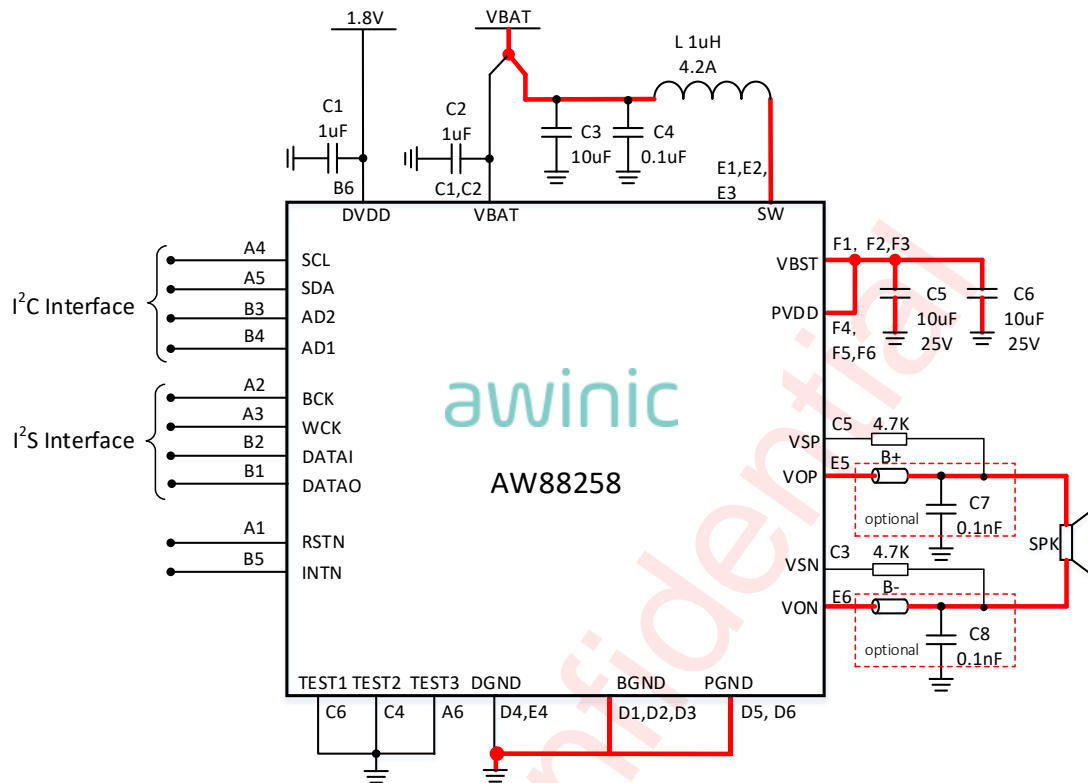
Figure 3 AW88258 Application Circuit
