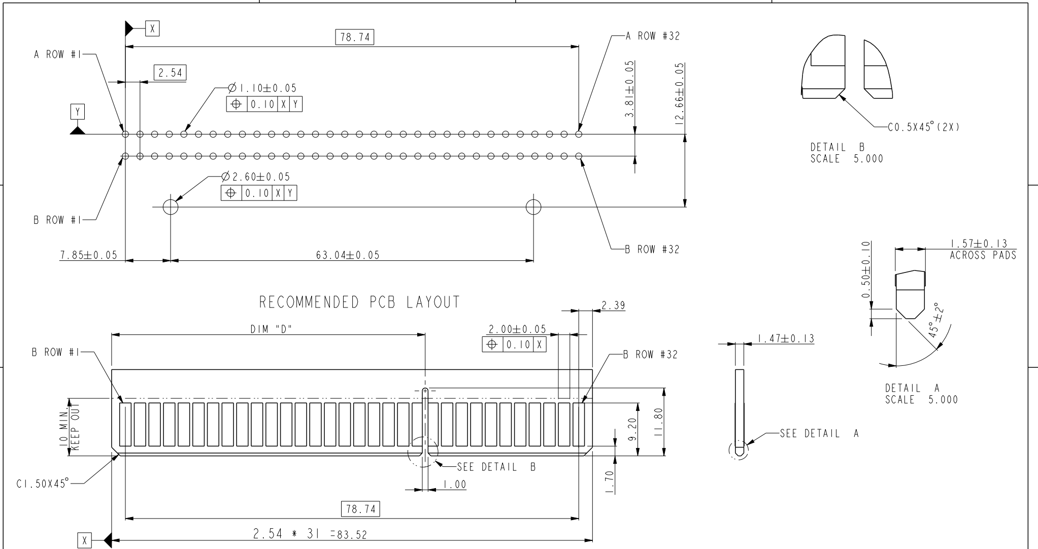
RECOMMENDED DAUGHTER CARD LAYOUT (TOP SIDE)
