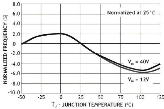
OSCILLATOR FREQUENCY
