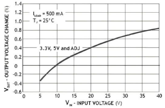
LINE REGULATION
