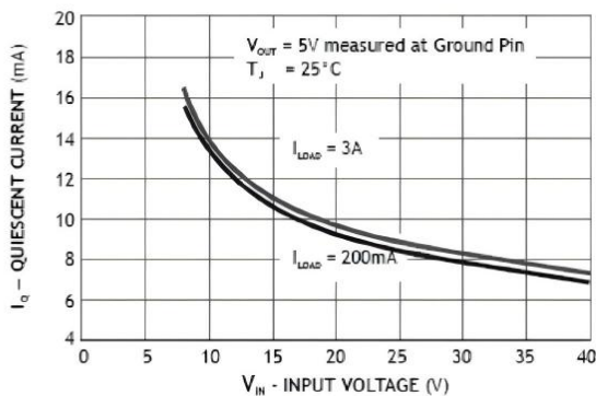
QUIESCENT CURRENT
