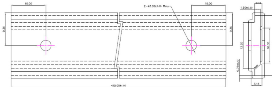
Figure 9b: Tube dimensions for L2C5-xxxx1202E0900.
