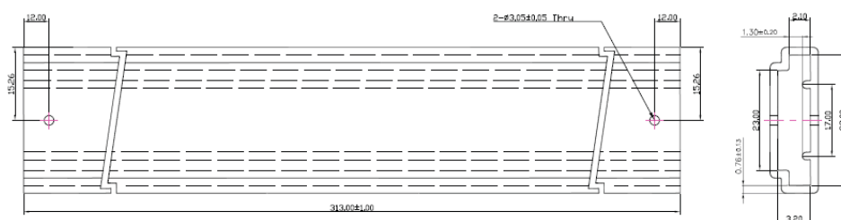
Figure 9d: Tube dimensions for L2C5-xxxx1211E1900 and L2C5-xxxx1216E2300.
