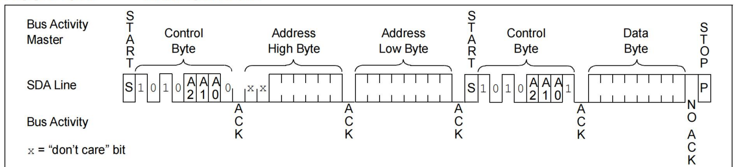
FIGURE 8-2: RANDOM READ
