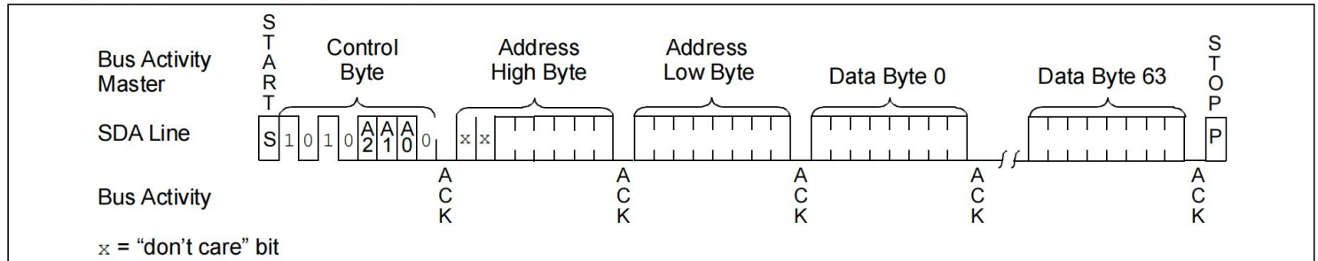
FIGURE 6-1: PAGE WRITE
