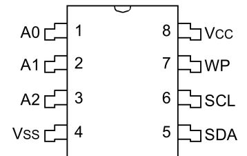
8-Lead SOIC/TSSOP (Top View)
