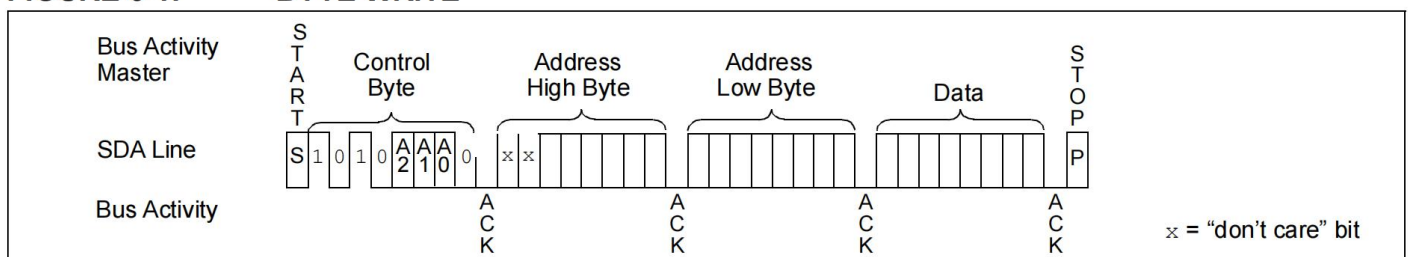
FIGURE 6-1: BYTE WRITE
