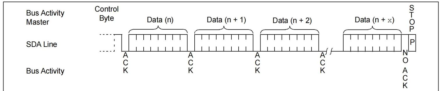
FIGURE 8-3: SEQUENTIAL READ
