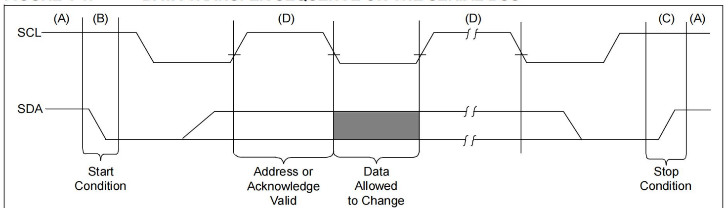
FIGURE 4-1: DATA TRANSFER SEQUENCE ON THE SERIAL BUS
