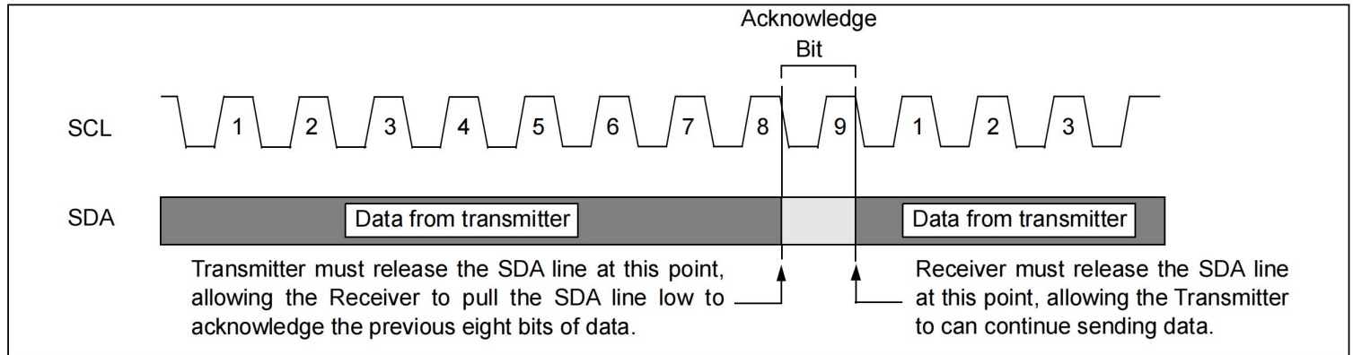
FIGURE 4-2: ACKNOWLEDGE TIMING
