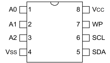
8-Lead PDIP (Top View)
